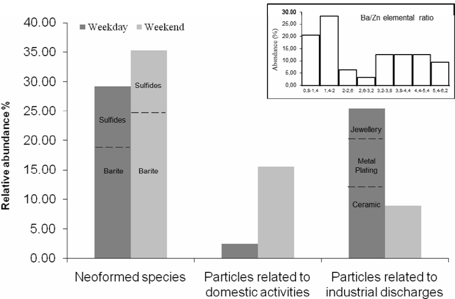
Figure 42: Relative abundance of heavy metal-bearing particles detected by backscattered electron imaging from (i) domestic activities, (ii) industrial wastes, and (iii) the sewer system. The inset shows the histogram of Ba/Zn elemental ratios in barite/sphalerite mixed particles.
