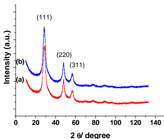
Figure 55. XRD peak patterns for (a) \text{ZnS}:\text{Mn}@ MPA and (b) \text{ZnS}:\text{Mn}@ MPA/ \text{ZnS} QDs.
