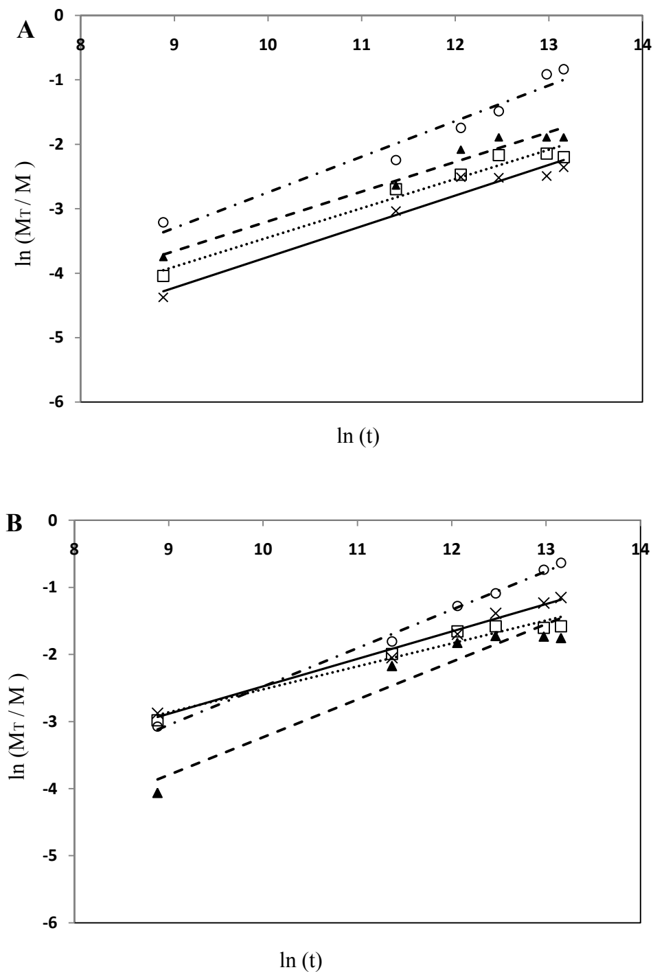
Figure 3: Curves of \ln(M_T/M) versus \ln(t) for active films containing nisin (0.137 mg nisin \text{cm}^{-2} ). ○, HPMC active film; ▲, chitosan active film; ×, sodium caseinate active film; and □ PLA active film at 4°C (A) and 40°C (B).
