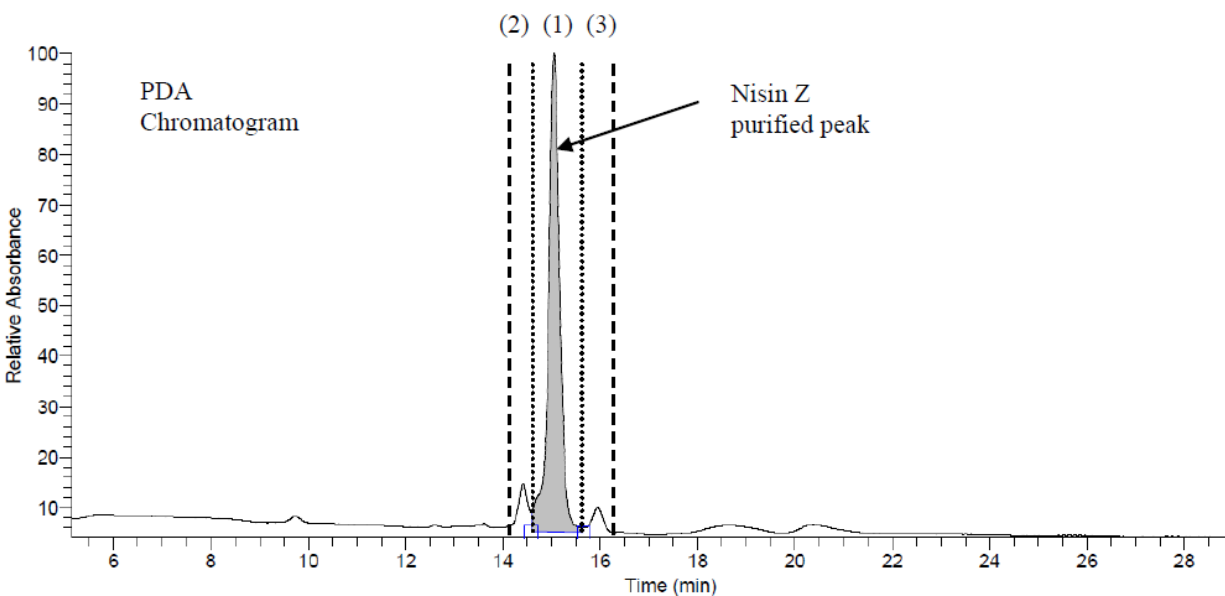
Figure 1: Purification of nisin Z major peak 1 by semi-preparative liquid chromatography. (1): nisin Z identified peak by LCMS detected as [M+3H]^{3+} ( m/z 1111.34) and [M+2H]^{2+} ( m/z 1666.33) ions (2, 3): tiny shoulder peaks of impurities corresponding to m/z 1116.66 and 1045.28 as [M+3H]^{3+} ions.
