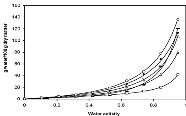
Fig. 1. Moisture sorption isotherms of HPMC, Nisaplin ® and glycerol composite films at 25 °C. Experimental DVS values were averaged and fitted by isotherm equation; solid lines represent the GAB model fitted to the data. (□) HPMC film, (Δ) HPMC + 30% glycerol, (X) HPMC + 50% glycerol, (—) HPMC + 10 4 IU Nisaplin ® , (◆) HPMC + 30% glycerol + 10 4 IU Nisaplin ® , (○) HPMC + 50% glycerol + 10 4 IU Nisaplin ® .
