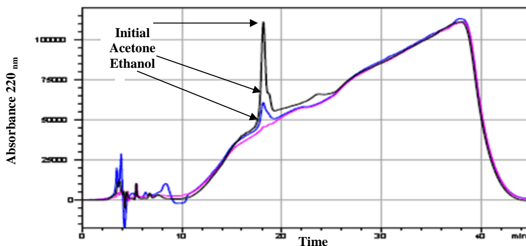
Figure 26. HPLC quantification under gradient elution and UV _{220\text{ nm}} detection of nisin 1 \text{g.L}^{-1} , nisin 1 \text{g.L}^{-1} after purification by acetone, and nisin 1 \text{g.L}^{-1} after purification by ethanol, injection 10 \mu\text{L} .
