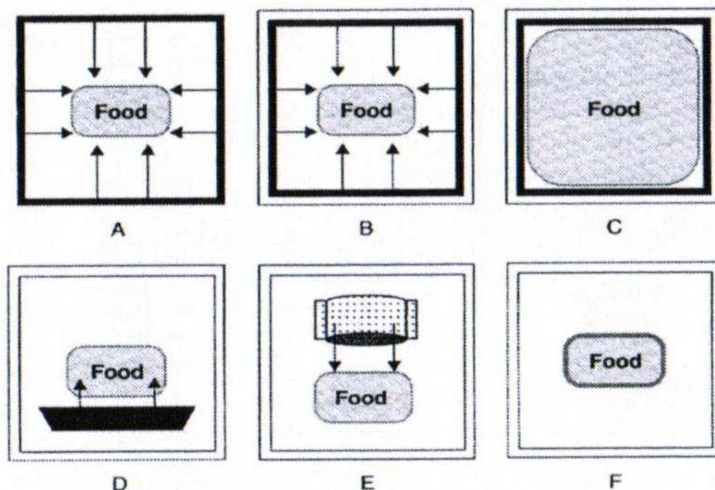
Figure 8. Possible ways to construct antimicrobial food packaging systems; A the use of antimicrobial packaging material; B antimicrobial coating on conventional packaging materials; C immobilization of antimicrobial agents in polymeric packaging materials; D the use of antimicrobial trays or pad; E the use of sachet or insert volatile antimicrobial agents; F antimicrobial edible coating on food (Han 2003).
