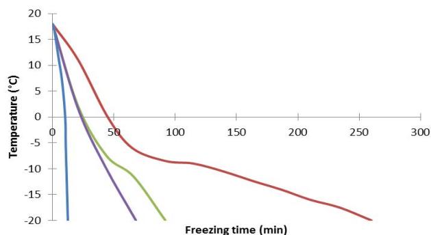
Fig. 1. Time-temperature history of sweet dough center at different freezing treatments: (—) 20\text{ }^{\circ}\text{C} , (—) 30\text{ }^{\circ}\text{C} , (—) 40\text{ }^{\circ}\text{C} and (—) liquid nitrogen.
