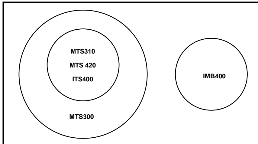
Figure 53. Crisp set
