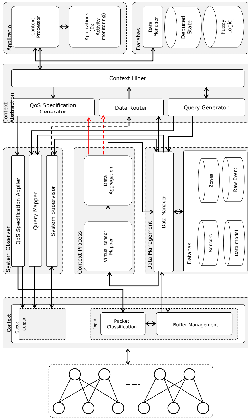
Figure 36. Modified architecture
