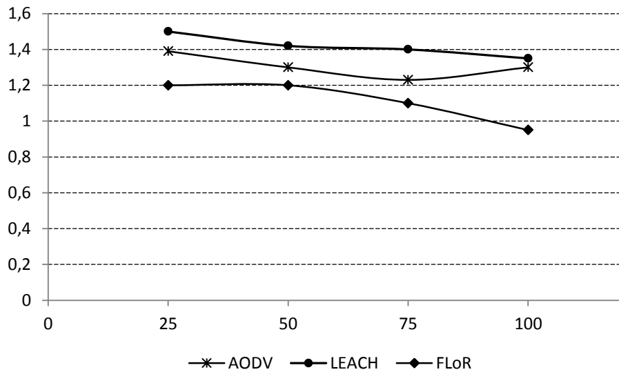
Figure 22. Routing overhead
