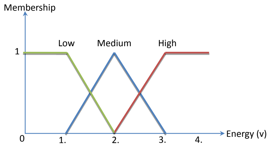
Figure 58. fuzzy membership function for battery energy
