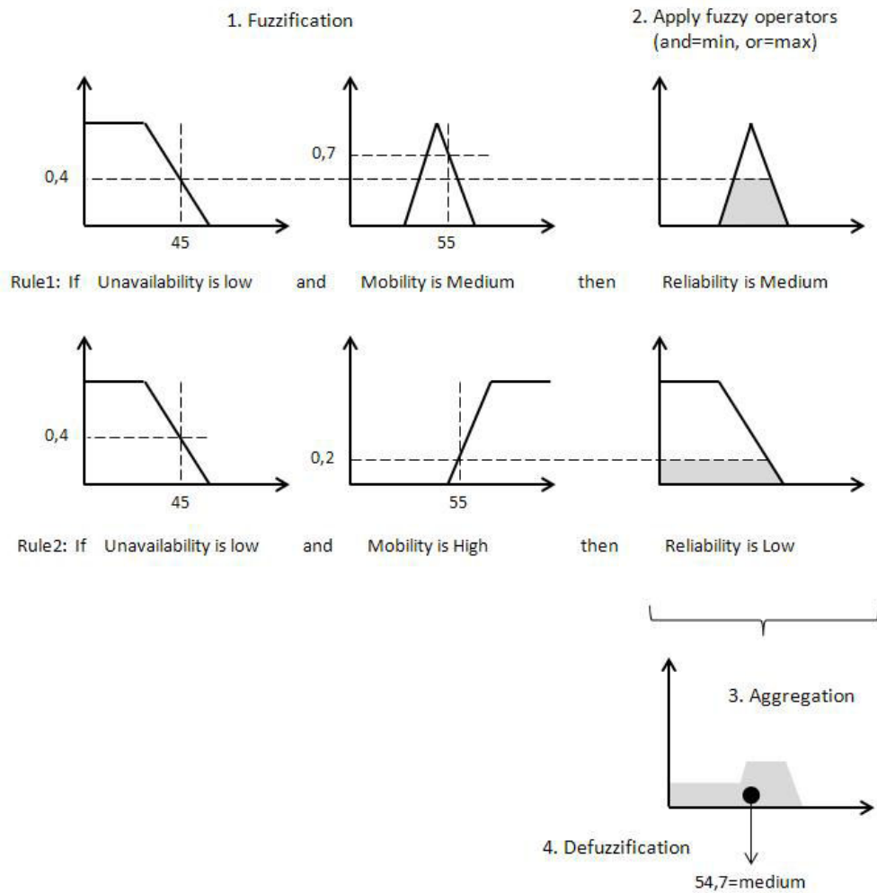
Figure 15. Fuzzy Inference Process
