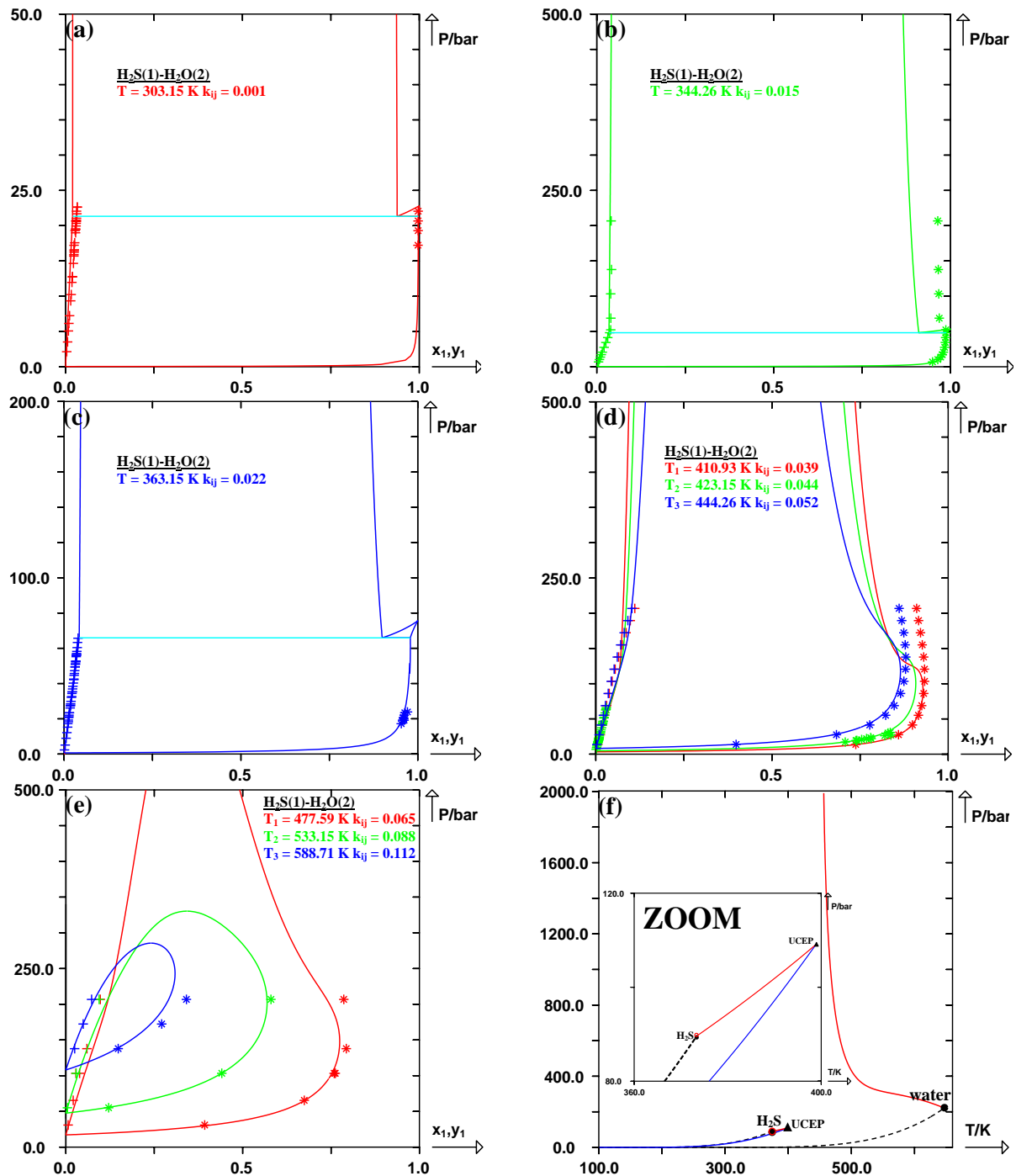
Figure II-18. Prediction of isothermal curves and prediction of the critical locus for the binary system: ( \text{H}_2\text{S}(1) + \text{H}_2\text{O}(2) ) using the PPR78 model. (+) experimental bubble points, (*) experimental dew points, (O) experimental critical points, (●) critical points of the pure compounds, (▲) upper critical endpoint, UCEP. Solid line: predicted curves with the PPR78 model. Dashed line: vaporization curve of the pure compounds. (a) System ( \text{H}_2\text{S}(1) + \text{H}_2\text{O}(2) ) at T = 303.15 \text{ K} ( k_{ij} = 0.001 ). (b) System ( \text{H}_2\text{S}(1) + \text{H}_2\text{O}(2) ) at T = 344.26 \text{ K} ( k_{ij} = 0.015 ). (c) System ( \text{H}_2\text{S}(1) + \text{H}_2\text{O}(2) ) at T = 363.15 \text{ K} ( k_{ij} = 0.022 ). (d) System ( \text{H}_2\text{S}(1) + \text{H}_2\text{O}(2) ) at three different temperatures: T_1 = 410.93 \text{ K} ( k_{ij} = 0.039 ), T_2 = 423.15 \text{ K} ( k_{ij} = 0.044 ), T_3 = 444.26 \text{ K} ( k_{ij} = 0.052 ). (e) System ( \text{H}_2\text{S}(1) + \text{H}_2\text{O}(2) ) at three different temperatures: T_1 = 477.59 \text{ K} ( k_{ij} = 0.065 ), T_2 = 533.15 \text{ K} ( k_{ij} = 0.088 ), T_3 = 588.71 \text{ K} ( k_{ij} = 0.112 ). (f) Critical locus of the system ( \text{H}_2\text{S}(1) + \text{H}_2\text{O}(2) ).
