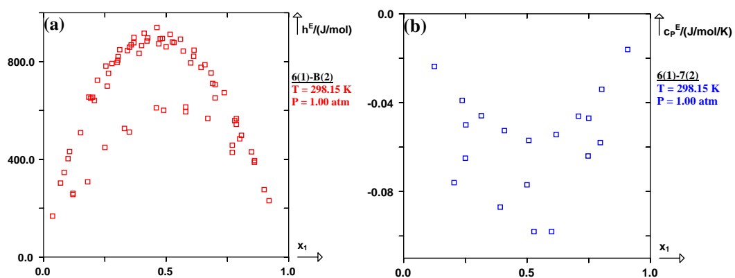
Figure V-2. (a) Experimental h^E points ( \square ) for the binary system (n-hexane(1) + benzene(2)) at T = 298.15 K and under one atmosphere ( P = 1.00 atm). (b) Experimental c_p^E points ( \square ) for the binary system (n-hexane(1) + n-heptane(2)) at T = 298.15 K and under one atmosphere ( P = 1.00 atm).
