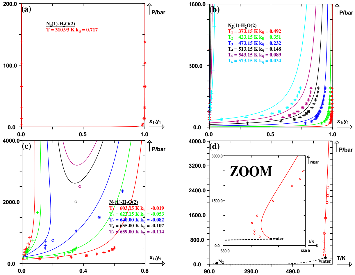
Figure II-17. Prediction of isothermal curves and prediction of the critical locus for the binary system: (N_2(1) + H_2O(2)) using the PPR78 model. (+) experimental bubble points, (*) experimental dew points, (○) experimental critical points, (●) critical points of the pure compounds. Solid line: predicted curves with the PPR78 model. Dashed line: vaporization curve of the pure compounds. (a) System (N_2(1) + H_2O(2)) at T = 310.93 \text{ K} ( k_{ij} = 0.717 ). (b) System (N_2(1) + H_2O(2)) at six different temperatures: T_1 = 373.15 \text{ K} ( k_{ij} = 0.492 ), T_2 = 423.15 \text{ K} ( k_{ij} = 0.351 ), T_3 = 473.15 \text{ K} ( k_{ij} = 0.232 ), T_4 = 513.15 \text{ K} ( k_{ij} = 0.148 ), T_5 = 543.15 \text{ K} ( k_{ij} = 0.089 ), T_6 = 573.15 \text{ K} ( k_{ij} = 0.034 ). (c) System (N_2(1) + H_2O(2)) at five different temperatures: T_1 = 603.15 \text{ K} ( k_{ij} = -0.019 ), T_2 = 623.15 \text{ K} ( k_{ij} = -0.053 ), T_3 = 640.00 \text{ K} ( k_{ij} = -0.082 ), T_4 = 655.00 \text{ K} ( k_{ij} = -0.107 ), T_5 = 659.00 \text{ K} ( k_{ij} = -0.114 ). (d) Critical locus of the system (N_2(1) + H_2O(2)) .
