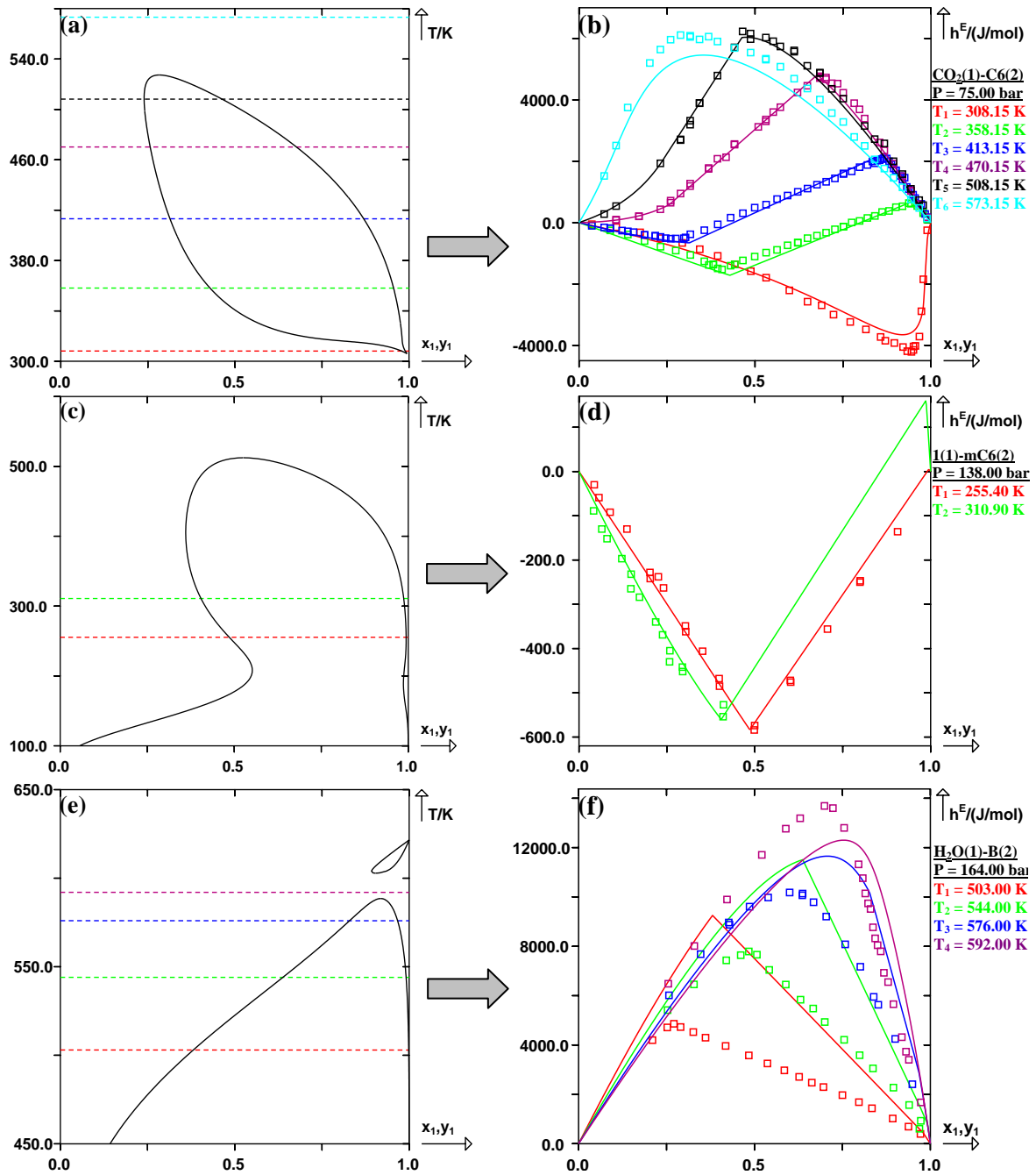
Figure V-26. Isobaric diagram and prediction of h^E curves referring to the two-phase region for three different binary systems: ( \text{CO}_2(1) + cyclohexane(2)), (methane(1) + methylcyclohexane(2)) and ( \text{H}_2\text{O}(1) + benzene(2)), using the E-PPR78 model. ( \square ) experimental h^E points. Solid line: predicted curves with the E-PPR78 model. Dashed line: constant temperature. (a) Isobaric curves for system ( \text{CO}_2(1) + cyclohexane(2)) under P = 75.00 bar. (b) h^E curves for system ( \text{CO}_2(1) + cyclohexane(2)) under P = 75.00 bar and at six different temperatures: T_1 = 308.15 K, T_2 = 358.15 K, T_3 = 413.15 K, T_4 = 470.15 K, T_5 = 508.15 K, T_6 = 573.15 K. (c) Isobaric curves for system (methane(1) + methylcyclohexane(2)) under P = 138.00 bar. (d) h^E curves for system (methane(1) + methylcyclohexane(2)) under P = 138.00 bar and at two different temperatures: T_1 = 255.40 K, T_2 = 310.90 K. (e) Isobaric curves for system ( \text{H}_2\text{O}(1) + benzene(2)) under P = 164.00 bar. (f) h^E curves for system ( \text{H}_2\text{O}(1) + benzene(2)) under P = 164.00 bar and at four different temperatures: T_1 = 503.00 K, T_2 = 544.00 K, T_3 = 576.00 K, T_4 = 592.00 K.
