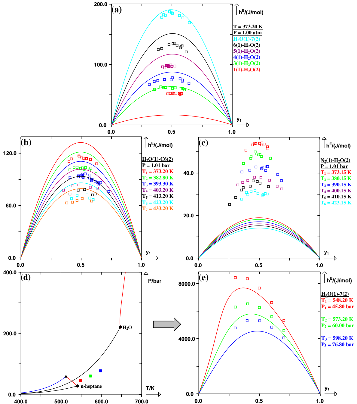
Figure V-19. Projection of pressure-temperature and prediction of h^E curves in the gaseous single-phase region for the binary systems containing H 2 O using the E-PPR78 model. (□) experimental h^E points, (■) pressure-temperature points, (●) critical points of the pure compounds, (▲) upper critical endpoint, UCEP. Solid line: predicted curves with the E-PPR78 model. (a) Six different systems at T = 373.20 \text{ K} and under one atmosphere ( P = 1.00 \text{ atm} ): (methane(1) + H 2 O(2)), (propane(1) + H 2 O(2)), (n-butane(1) + H 2 O(2)), (n-pentane(1) + H 2 O(2)), (n-hexane(1) + H 2 O(2)), (H 2 O(1) + n-heptane(2)). (b) System (H 2 O(1) + cyclohexane(2)) under P = 1.01 \text{ bar} and at seven different temperatures: T_1 = 373.20 \text{ K} , T_2 = 382.80 \text{ K} , T_3 = 393.30 \text{ K} , T_4 = 403.20 \text{ K} , T_5 = 413.20 \text{ K} , T_6 = 423.20 \text{ K} , T_7 = 433.20 \text{ K} . (c) System (N 2 (1) + H 2 O(2)) under P = 1.01 \text{ bar} and at six different temperatures: T_1 = 373.15 \text{ K} , T_2 = 380.15 \text{ K} , T_3 = 390.15 \text{ K} , T_4 = 400.15 \text{ K} , T_5 = 410.15 \text{ K} , T_6 = 423.15 \text{ K} . (d) Pressure-temperature projection for system (H 2 O(1) + n-heptane(2)) with the pressure-temperature points where the h^E curves are predicted. (e) System (H 2 O(1) + n-heptane(2)) at: T_1 = 548.20 \text{ K} and P_1 = 45.80 \text{ bar} , T_2 = 573.20 \text{ K} and P_2 = 60.00 \text{ bar} , T_3 = 598.20 \text{ K} and P_3 = 76.80 \text{ bar} .
