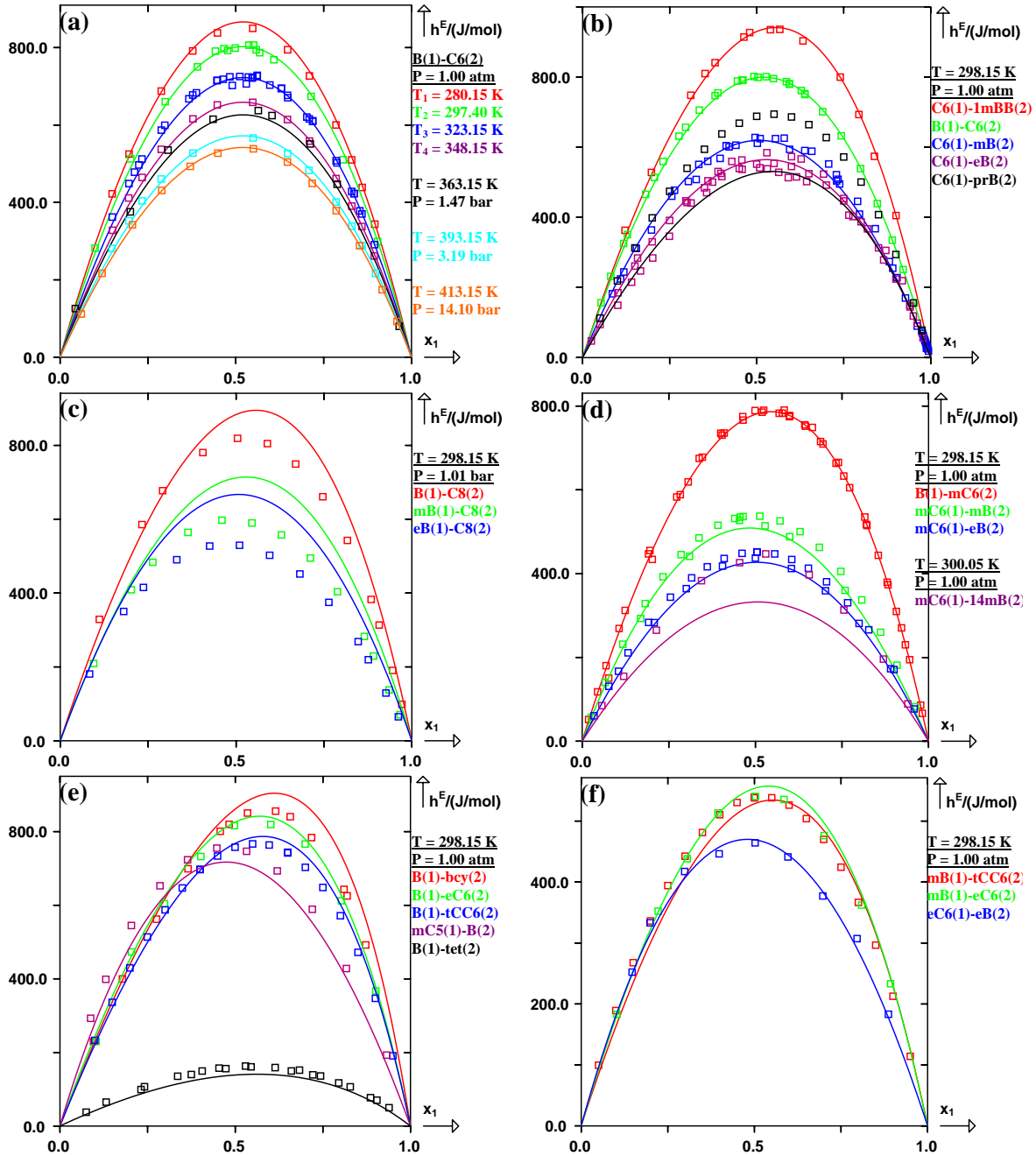
Figure V-11. Prediction of h^E curves in the liquid single-phase region for the binary systems consist of a naphthene and an aromatic using the E -PPR78 model. ( \square ) experimental h^E points. Solid line: predicted curves with the E -PPR78 model. (a) System (benzene(1) + cyclohexane(2)) under one atmosphere ( P = 1.00 atm) and at four different temperatures: T_1 = 280.15 K, T_2 = 297.40 K, T_3 = 323.15 K, T_4 = 348.15 K, under P = 1.47 bar and at T = 363.15 K, under P = 3.19 bar and at T = 393.15 K, under P = 14.10 bar and at T = 413.15 K. (b) Five different systems at T = 298.15 K and under one atmosphere ( P = 1.00 atm): (cyclohexane(1) + 1-methylnaphthalene(2)), (benzene(1) + cyclohexane(2)), (cyclohexane(1) + toluene(2)), (cyclohexane(1) + ethylbenzene(2)), (cyclohexane(1) + n-propylbenzene(2)). (c) Three different systems at T = 298.15 K and under P = 1.01 bar: (benzene(1) + cyclooctane(2)), (toluene(1) + cyclooctane(2)), (ethylbenzene(1) + cyclooctane(2)). (d) Three different systems at T = 298.15 K and under one atmosphere ( P = 1.00 atm): (benzene(1) + methylcyclohexane(2)), (methylcyclohexane(1) + toluene(2)), (methylcyclohexane(1) + ethylbenzene(2)), one system at T = 300.05 K and under one atmosphere ( P = 1.00 atm): (methylcyclohexane(1) + 1,4-dimethylbenzene(2)). (e) Five different systems at T = 298.15 K and under one atmosphere ( P = 1.00 atm): (benzene(1) + 1,1'-bicyclohexyl(2)), (benzene(1) + ethylcyclohexane(2)), (benzene(1) + trans-decalin(2)), (methylcyclopentane(1) + benzene(2)), (benzene(1) + tetralin(2)). (f) Three different systems at T = 298.15 K and under one atmosphere ( P = 1.00 atm): (toluene(1) + trans-decalin(2)), (toluene(1) + ethylcyclohexane(2)), (ethylcyclohexane(1) + ethylbenzene(2)).
