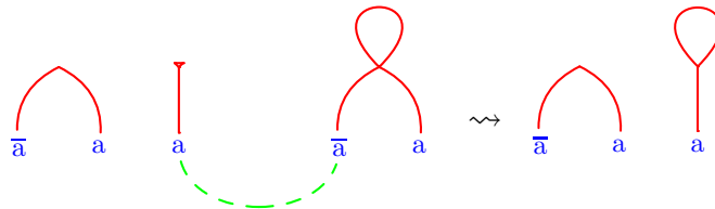
FIGURE 4.2 – Cut elimination performed on two CL-correct F-nets that results in an F-prenet not corresponding to a CL proof.
