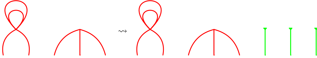
FIGURE 3.16 – \uparrow transformation on a linking
