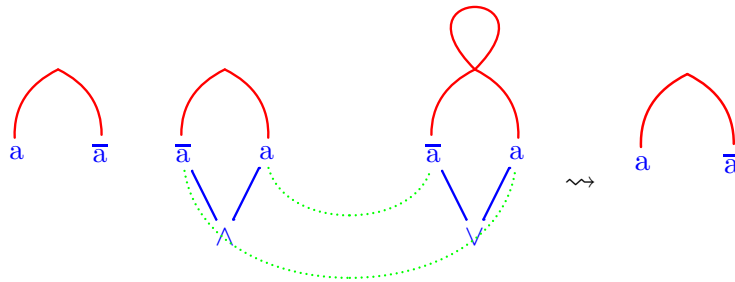
FIGURE 4.6 – Cut elimination can remove components altogether. This corresponds to the thinness property of Frobenius algebras.
