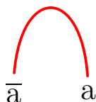
FIGURE 3.19 – F-prenet for the Ax rule
