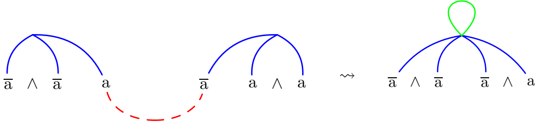
FIGURE 4.4 – Cut elimination on FL-correct F-nets does not yield an FL-correct F-net. The green loop that is added is required to get an FL-correct net, but is not obtained from the composition.
