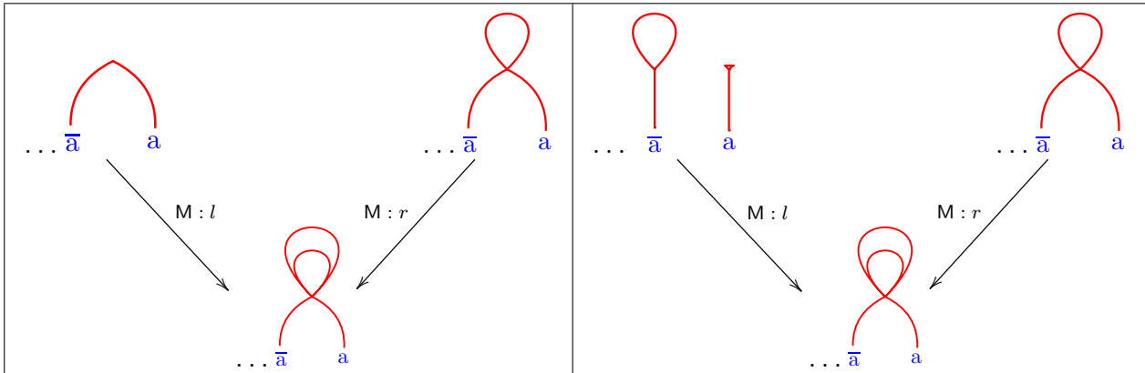
FIGURE 3.27 – Two different (elementary) M -cospans with a common leg.
