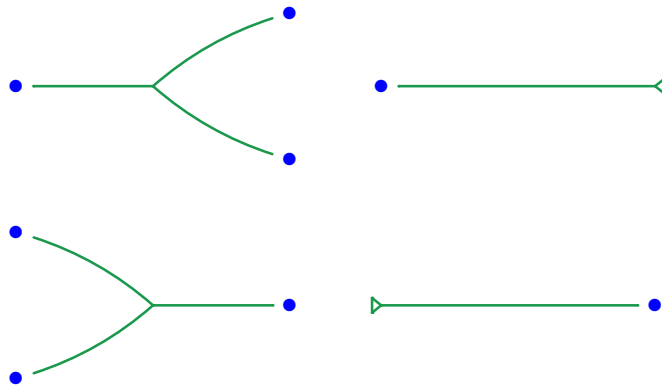
FIGURE 3.5 – Generators in the category FrFrob – up : comonoid comultiplication \Delta (diagonal) and counit \Pi (projection); down : monoid multiplication \nabla (co-diagonal) and unit \Pi (co-projection). Notice the use of a 'terminator' triangle symbol in (co)unit generators to denote the single graph vertex that is not an object generator.
