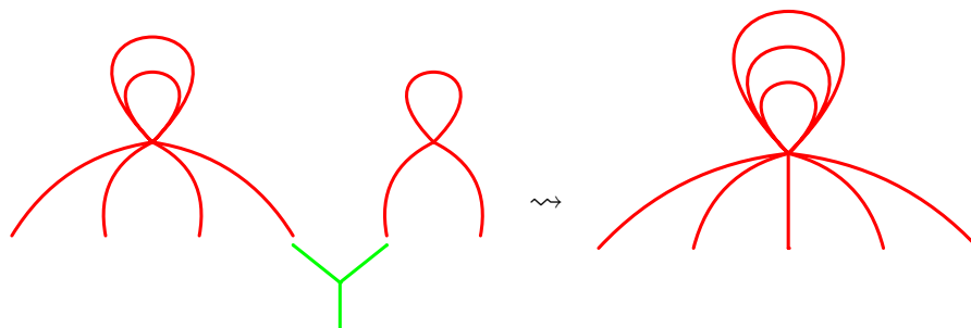
FIGURE 3.13 – \gamma_d transformation on a linking
