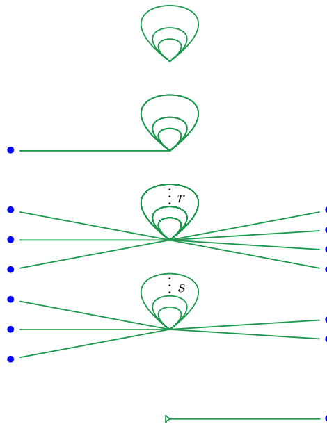
FIGURE 3.4 – A map in the category \mathbf{FrFrob} as a collection of wires between endpoints with loops, depicted horizontally. Notice that it is possible for a component not to be connected to any endpoint and notice how we use the 'terminator' symbol to denote the base-point with no loops, connected to a single endpoint.
