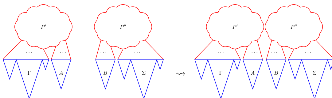
FIGURE 3.22 – F-prenet for the Mix rule. Notice how this rule is 'invisible' from the point of view of F-prenet representations.
