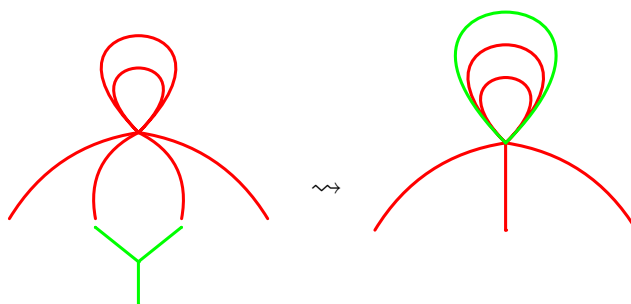
FIGURE 3.12 – \gamma_s transformation on a linking
