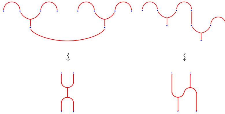
FIGURE 4.1 – F-nets for proofs on Figure 3.10 identified by the Frobenius axiom.
