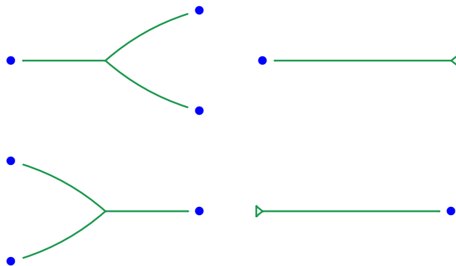
FIGURE 3.5 – Generators in the category FrFrob – up : comonoid comultiplication \Delta (diagonal) and counit \Pi (projection); down : monoid multiplication \nabla (co-diagonal) and unit I (co-projection). Notice the use of a 'terminator' triangle symbol in (co)unit generators to denote the single graph vertex that is not an object generator.
