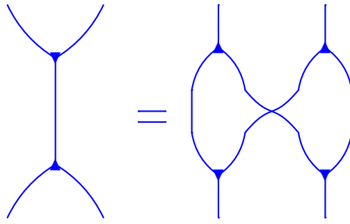
FIGURE 3.9 – Bialgebra equation
