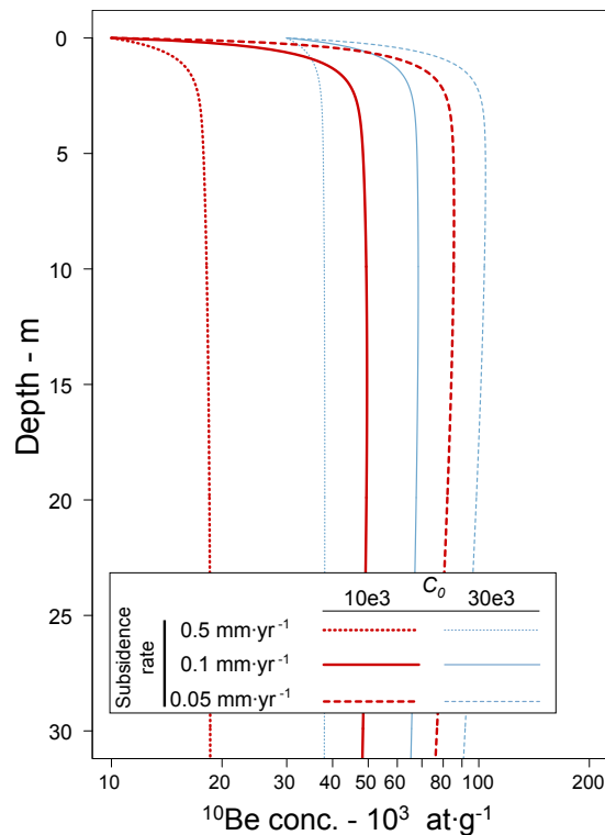
Figure IV.18: Evolution of ^{10}\text{Be} concentration in a soil profile under steady state subsidence ( 0.5 , 0.1 and 0.05 \text{mm}\cdot\text{yr}^{-1} ) accommodated by sediments of constant concentration of 10\cdot 10^3 \text{at}\cdot\text{g}^{-1} (red) and 30\cdot 10^3 \text{at}\cdot\text{g}^{-1} (blue). Floodplain storage of Himalayan sediments systematically leads to an increase in ^{10}\text{Be} concentration. (Floodplain production rate: 4.6 \text{at}\cdot\text{g}^{-1}\cdot\text{yr}^{-1} and soil density 2 \text{g}\cdot\text{cm}^{-3} ).
