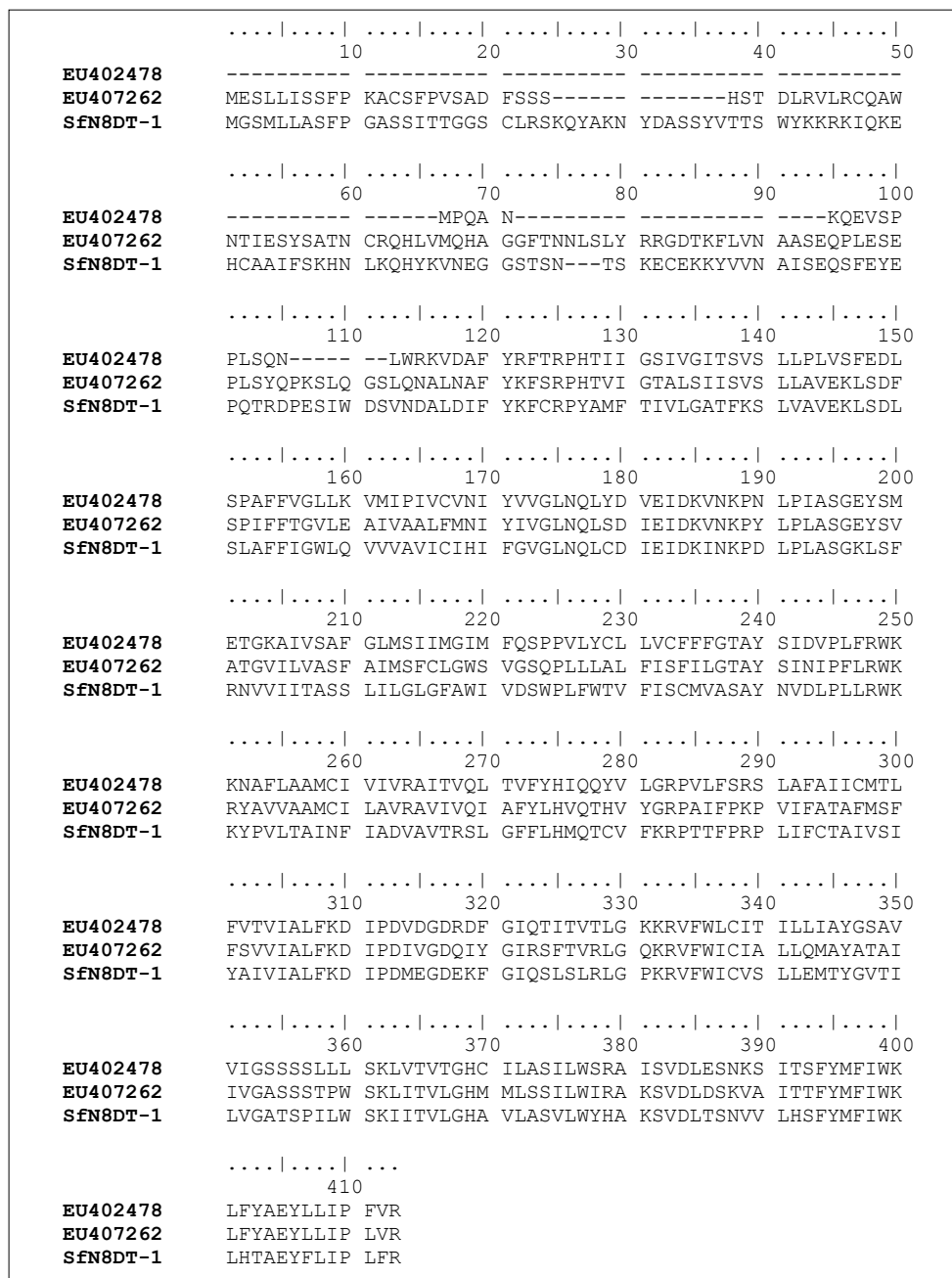
Figure 60. Alignment of the peptidic sequence of EU402478, EU407262 and SfN8DT-1
