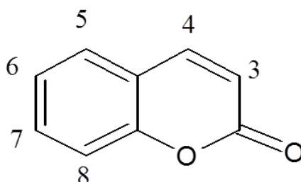
Figure 3. Basic structure of coumarins
