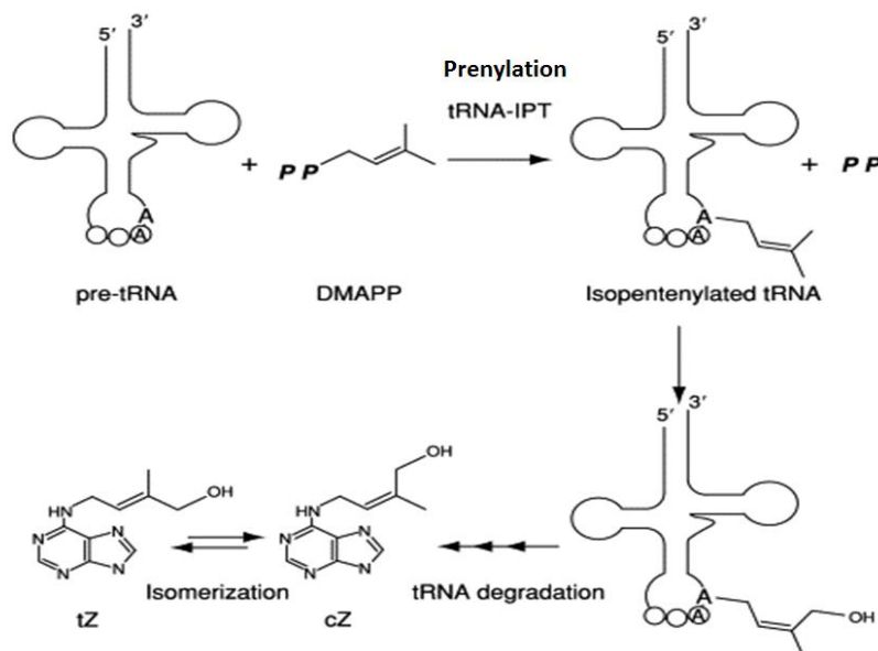
Figure 23. Hypothesized pathway for tRNA-mediated cis-Zeatin biosynthesis
