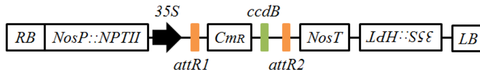
Figure 47. T-DNA region of plasmid pGWB2
