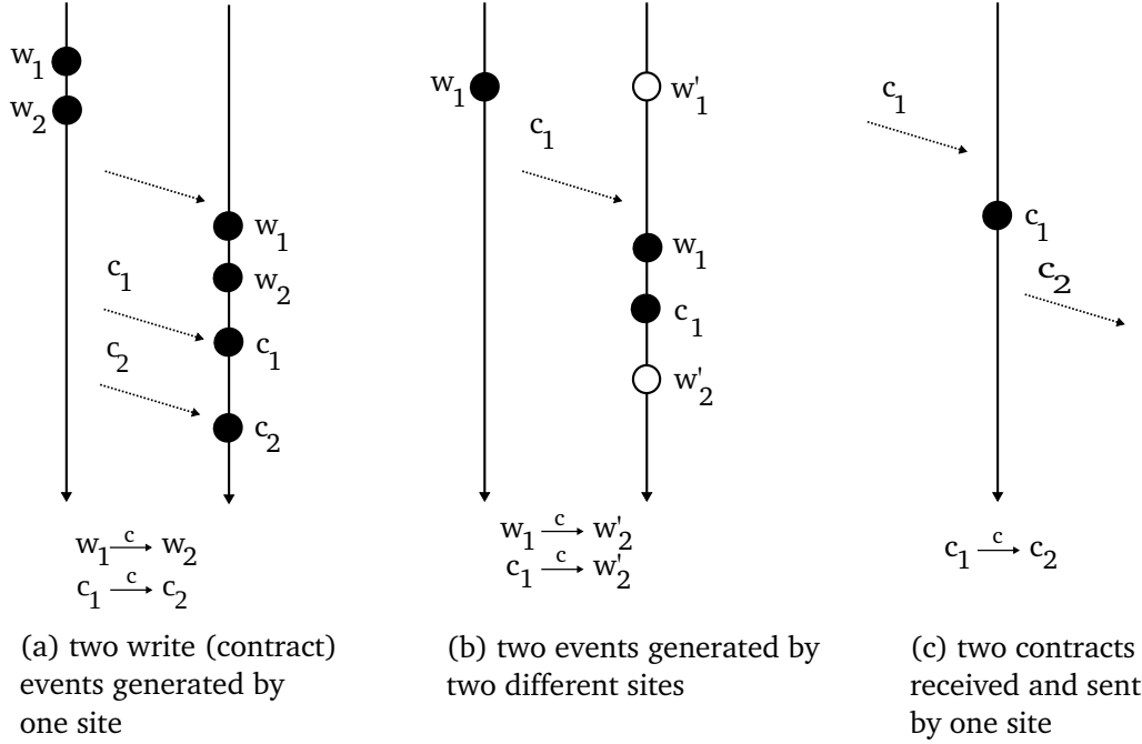
Figure 4.11. Causal relations between events ( w_i represents for write events and c_i represents for contract or communication events).
