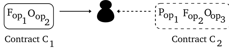
Figure 4.10. A scenario when a user adopts two contracts that are inconsistent. The user holds Contract 1 and a coming one Contract 2. The conflict between O_{op_2} and F_{op_2} needs to be resolved to proceed further actions.
