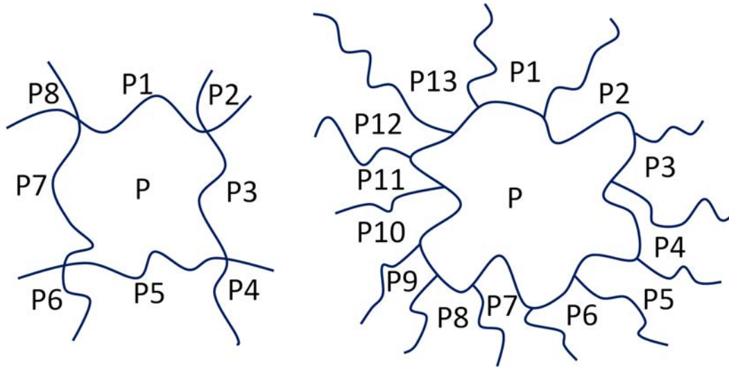
Figure 5.18: Surrounding patches in case of the structured synthesizer and the stochastic synthesizer. Left : In the structured synthesizer, the number of surrounding patches is 8. Right : In the stochastic synthesizer, the number of surrounding patches is arbitrary. When the number of surrounding patches is high, filtering artifacts may occur under minification.
