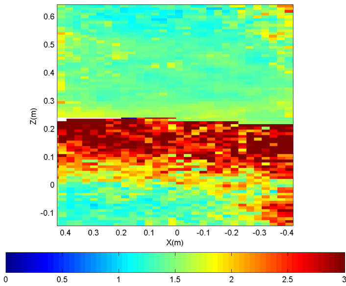
Figure VI.19 – Mesures PIV, \overline{u'^2}/(R\omega/100) (Plan axial Y=0 , 500 \text{tr.min}^{-1} )
