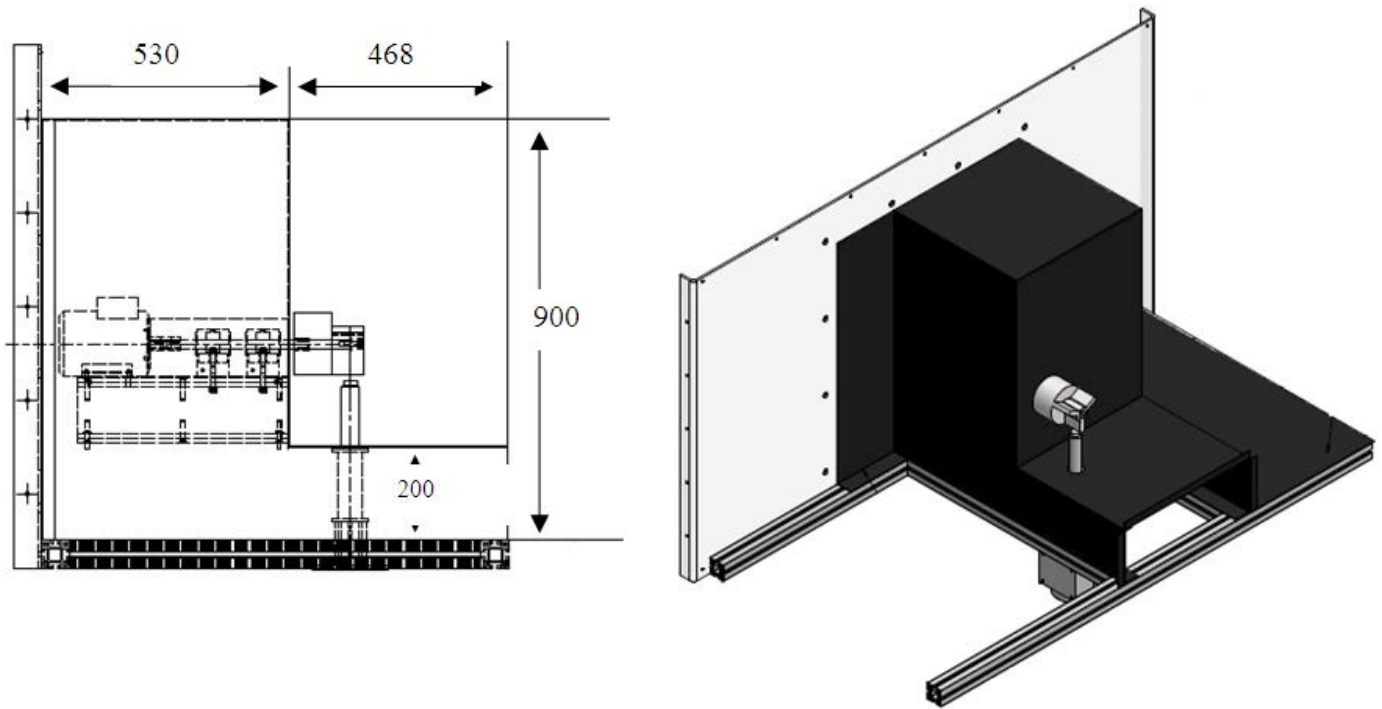
Figure II.11 – Capotage (mm)
