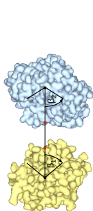
Fig. 3. Illustration of an initial docking pose between a pair of candidate SH domains. The angles \beta_1 and \beta_2 represent the Hes docking search range angles which will be applied to focus the docking search around the putative interface. Black spheres represent the centre of mass of each domain, and red spheres represent the central residue of each binding site.
