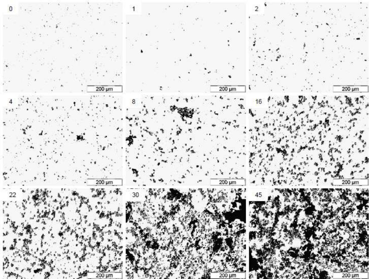
Fig. 3. Optical microscopy pictures of biofilms on glass coupons from day 0 to day 45 at 42°C (R1-42). The number at the top-left indicates the time in days.
