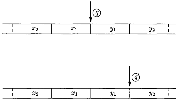
Figure 5.1: A “move right” Node
