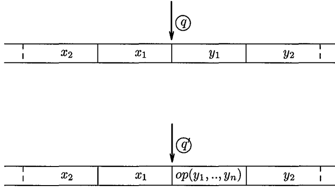
Figure 6.2: An “op” Node
