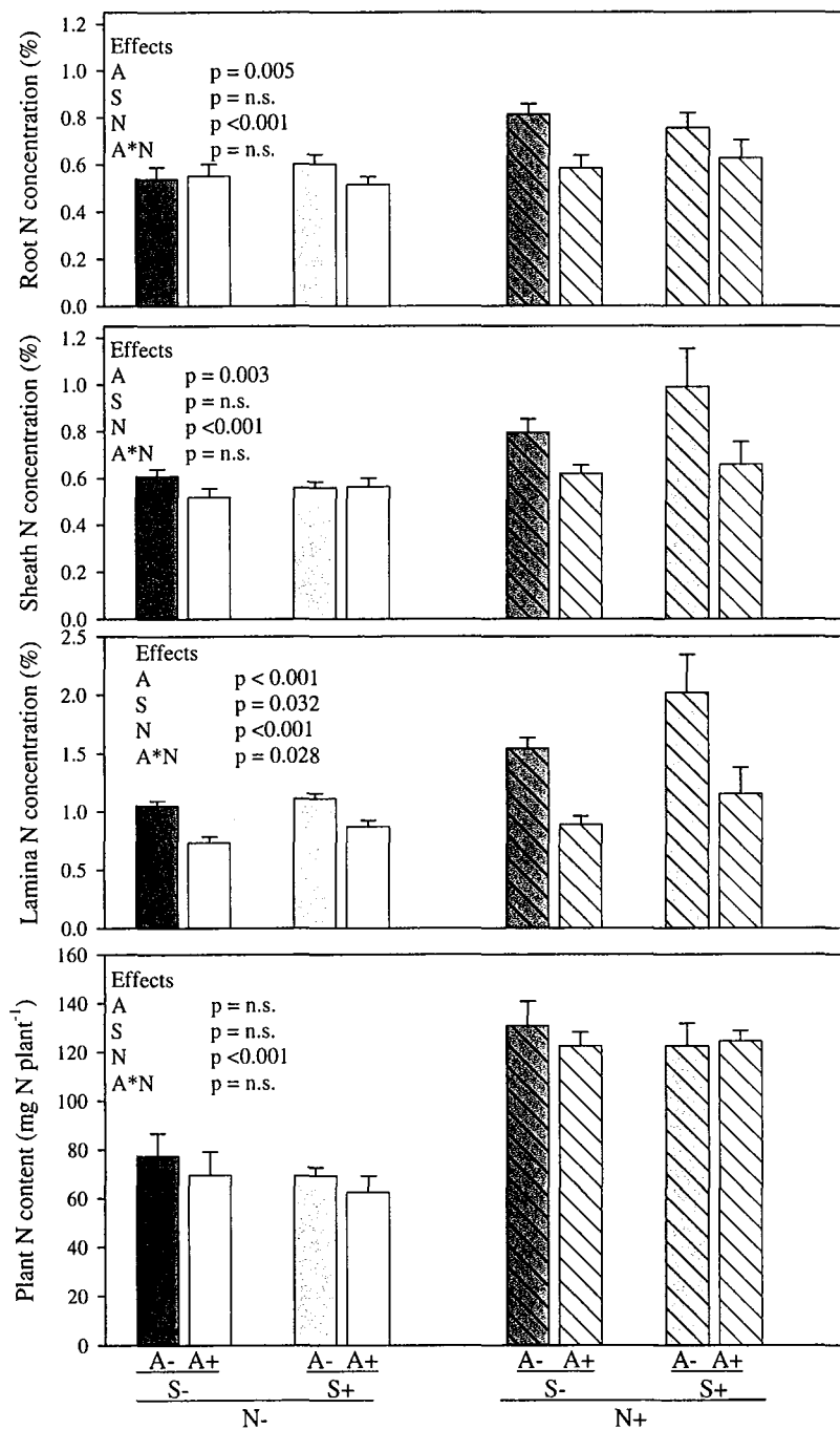
Figure 5.4: Effects of the treatment on root, stem and leaf N concentration (%) and total plant N content (mg N plant -1 ). Values are average of 6 replicates \pm SE. Bars are grouped by fertiliser N (low, N- or high, N+), soil type (ambient soil, S- or enriched soil, S+) and atmospheric CO 2 concentration (ambient, A- or enriched, A+). P values are given for the main effects
