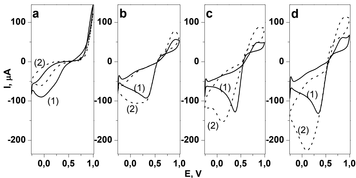
Fig. 4.19. Response of Pt-NPs modified non-macroporous CNT layers (1) and macroporous CNT layers ( [PS\ beads] = 0.2\ mg/mL ) (2) to 10\ mM\ H_2O_2 . Time of electrophoretic deposition: (a) 15 s, (b) 45 s, (c) 75 s, (d) 105 s; supporting electrolyte: 0.1M\ H_2SO_4 ; scan rate: 10\ mV/s .
