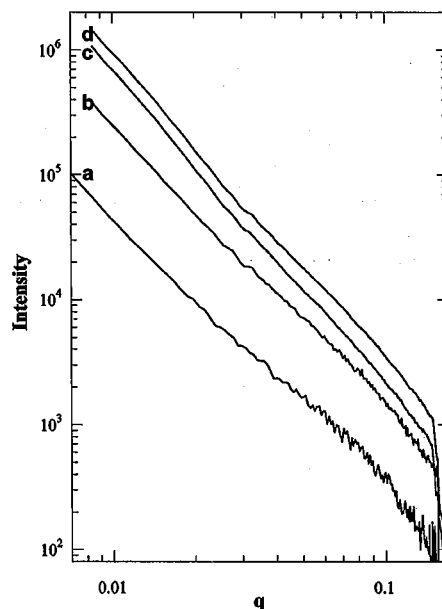
Figure 3. Experimental SAXS curves of colloids obtained at various hydrolysis ratios: (a) R = 0.7 ; (b) R = 0.9 ; (c) R = 1.4 ; and (d) R = 2.0 .
