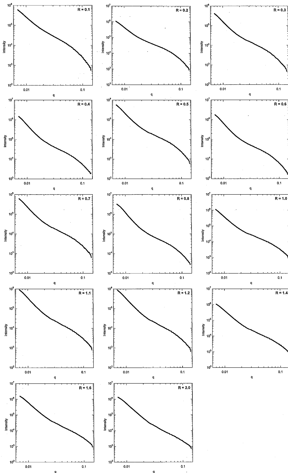
Figure 7. Experimental small-angle X-ray scattering curves of colloids obtained at various hydrolysis ratios.
