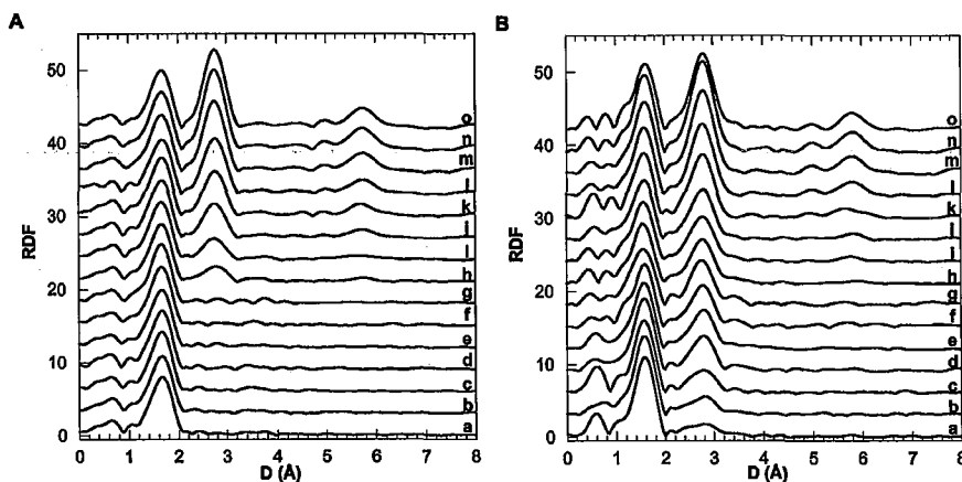
Figure 8. Nickel and Gallium RDFs (uncorrected for phase shifts) for mixed nickel-gallium chloride solutions at various hydrolysis ratios R = [\text{OH}^-]/[\text{Ni}^{2+} + \text{Ga}^{3+}] : (A) Ni K edge; (B) Ga K edge. (a) R = 0.2 , (b) R = 0.3 , (c) R = 0.4 , (d) R = 0.6 , (e) R = 0.7 , (f) R = 0.8 , (g) R = 0.9 , (h) R = 1.0 , (i) R = 1.1 , (j) R = 1.2 , (k) R = 1.4 , (l) R = 1.6 , (m) R = 1.8 , (n) R = 2.0 , (o) R = 2.4 .
