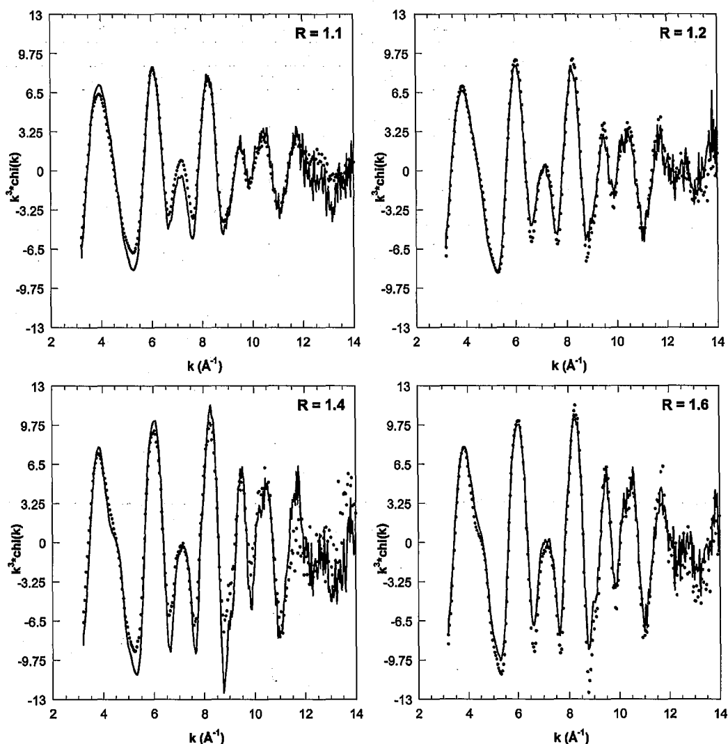
Figure 10. Comparison between filtered Ga K-edge EXAFS spectra of mixed nickel-gallium chloride solutions at various R values and linear combinations of GaOOH spectra and NiGa LDH spectra. The proportions of the LDH phase in the solids are reported in Table 5. Solid line: experimental spectrum. Dotted line: calculated spectrum.
