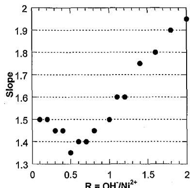
Figure 8. Evolution of the slopes of the experimental curves at high q values as a function of hydrolysis ratio.
