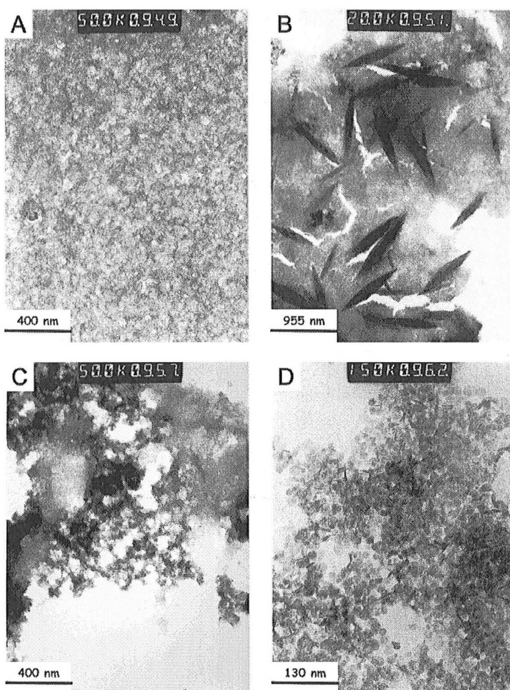
Figure 5. TEM micrographs of aged colloidal suspensions for various R values: (A) R = 0.9 ; (B) R = 1.1 ; (C) R = 1.4 ; and (D) R = 2.0 .
