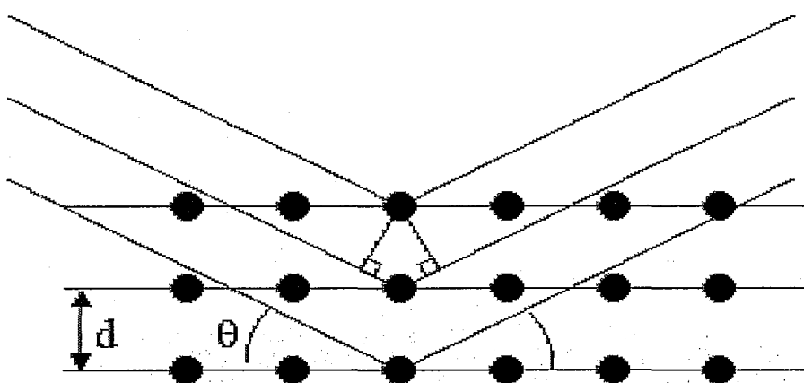
Figure 6 : Condition de Bragg
