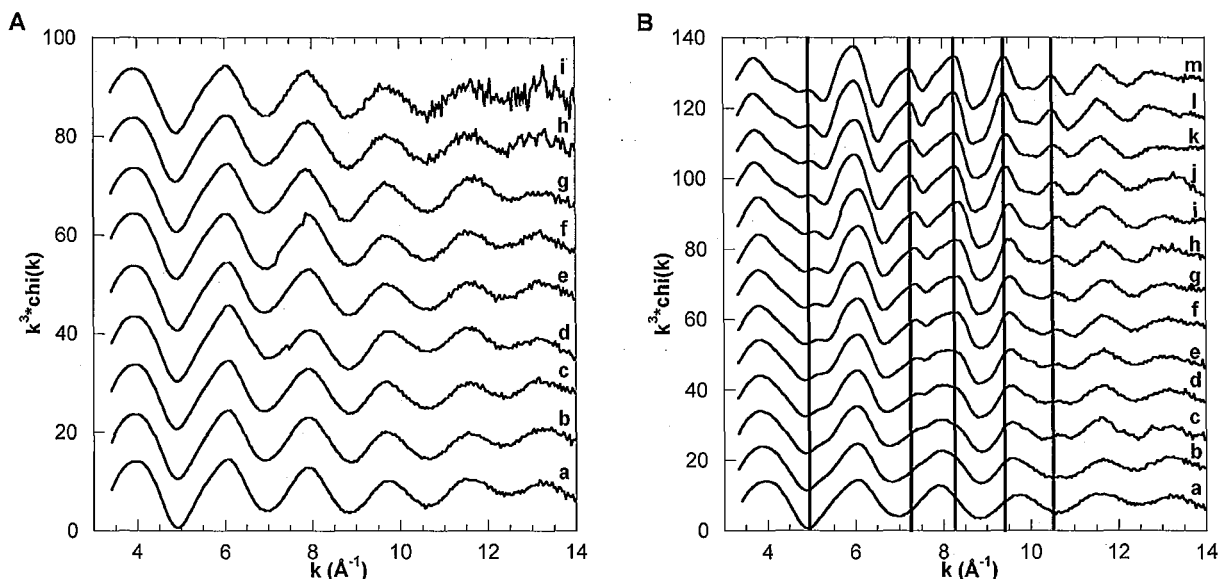
Figure 2. Ni EXAFS spectra for nickel chloride solutions at various hydrolysis ratios, R = \text{OH}^-/\text{Ni}^{2+} : A, supernatant; B, colloids; a, R = 0.0 ; b, R = 0.1 ; c, R = 0.2 ; d, R = 0.4 ; e, R = 0.6 ; f, R = 0.8 ; g, R = 1.0 ; h, R = 1.2 ; i, R = 1.4 ; j, R = 1.6 ; k, R = 1.7 ; l, R = 1.8 ; m, R = 2.0 .
