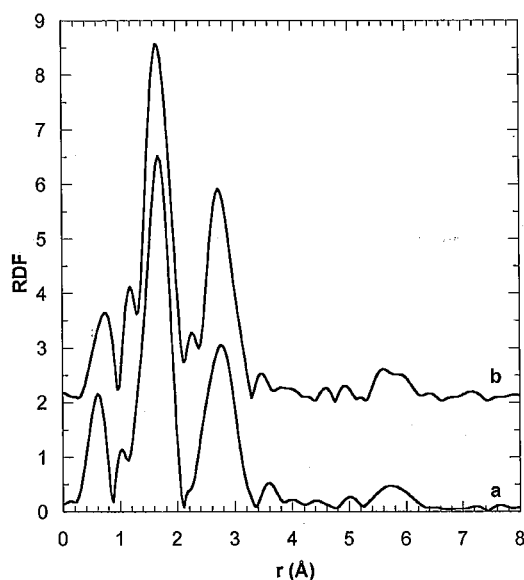
Figure 6. Nickel RDFs (uncorrected for phase shifts) for nickel chloride solutions at various hydrolysis ratios R = \text{OH}^-/\text{Ni}^{2+} after centrifugation of the colloidal suspension: a, R = 0.1 ; b, R = 0.2 .
