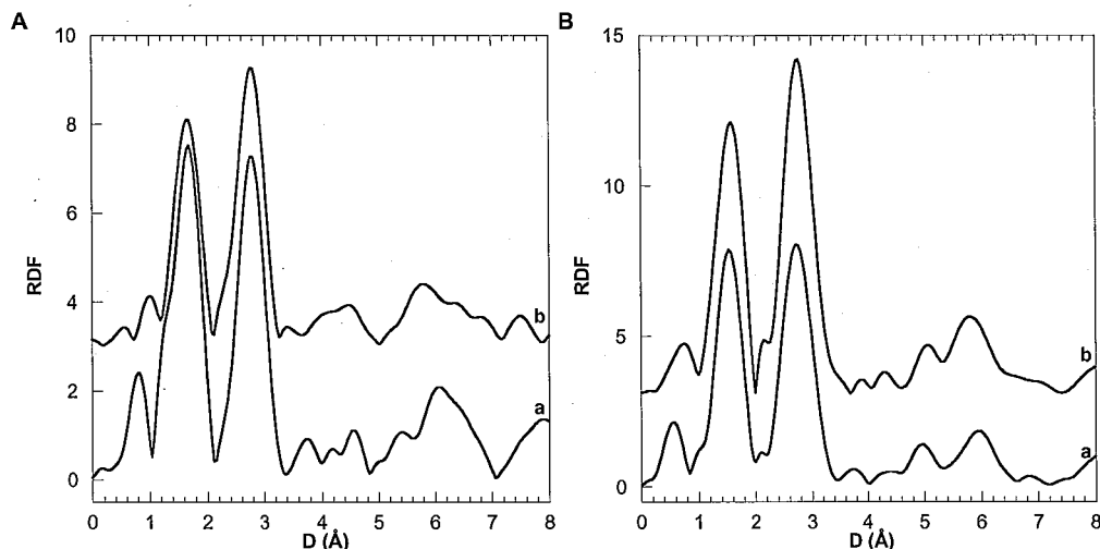
Figure 10. Ni and Ga K-edge RDFS obtained on the centrifuged colloids synthesized from mixed nickel-gallium ( Ni/Ga = 4 ) chloride solution at various salt solution volumes V_s :
