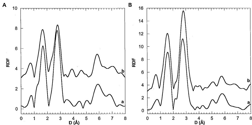
Figure 11. Ni and Ga K-edge RDFS obtained on the centrifuged colloids synthesized from mixed nickel-gallium ( Ni/Ga = 6 ) chloride solution at various salt solution volumes V_s :
