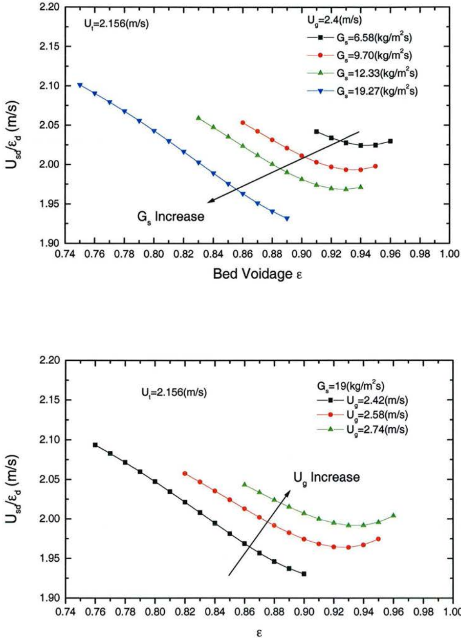
Fig. 5-8 Real Slip Velocity in Dilute Phase at Different U_g and G_s
