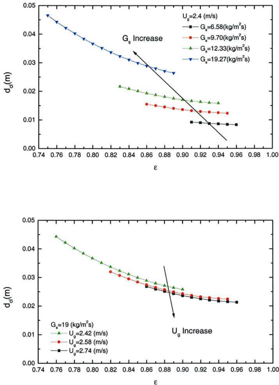
Fig. 5-12 Relation Between d_{cl} and \varepsilon at Different U_g and G_s
