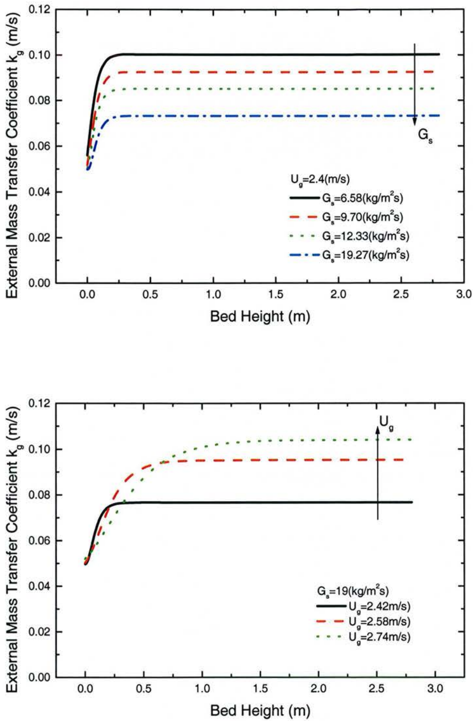
Fig. 6-5 The Changes of External Mass Transfer Coefficient along the Bed Height under Various Operating Conditions
