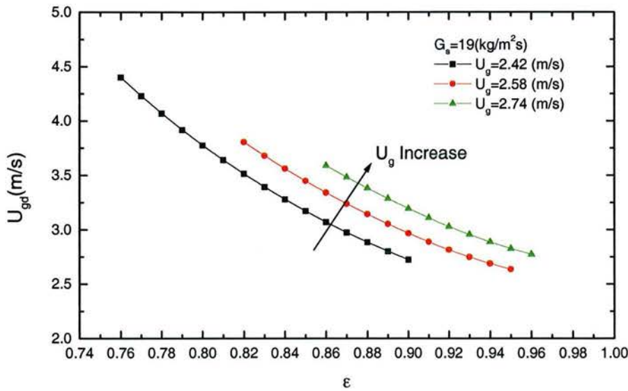
Fig. 5-5 Relation Between U_{gd} and \epsilon at Different U_g and G_s
