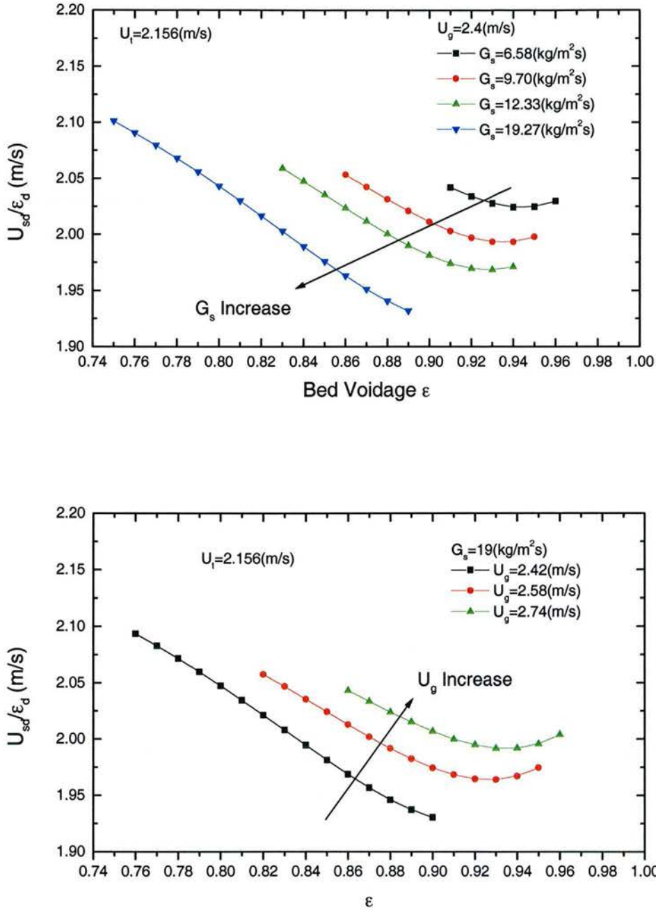
Fig. 5-8 Real Slip Velocity in Dilute Phase at Different U_g and G_s
