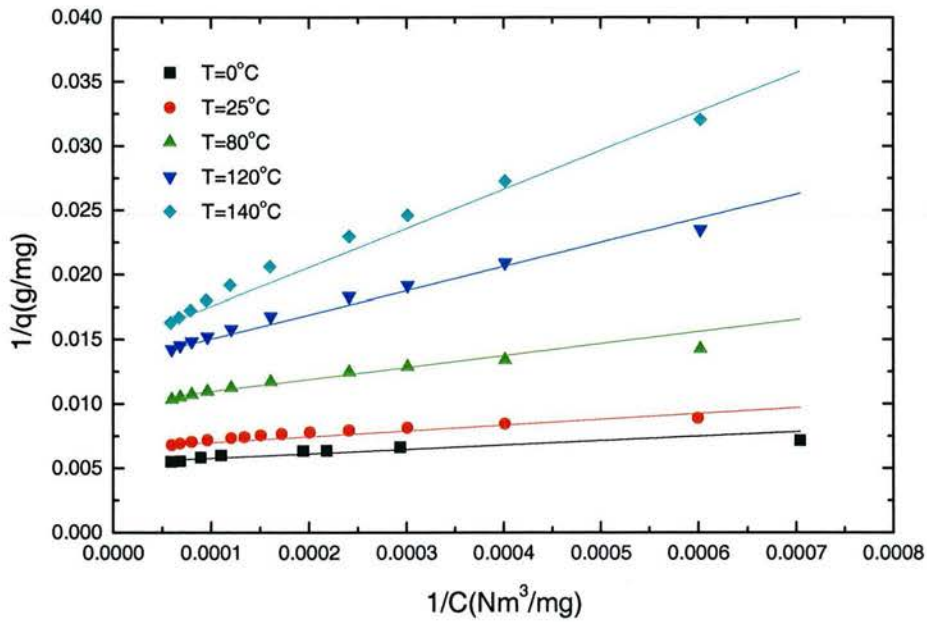
Fig. 2-5 Experimental data fitted with Langmuir Isotherm
