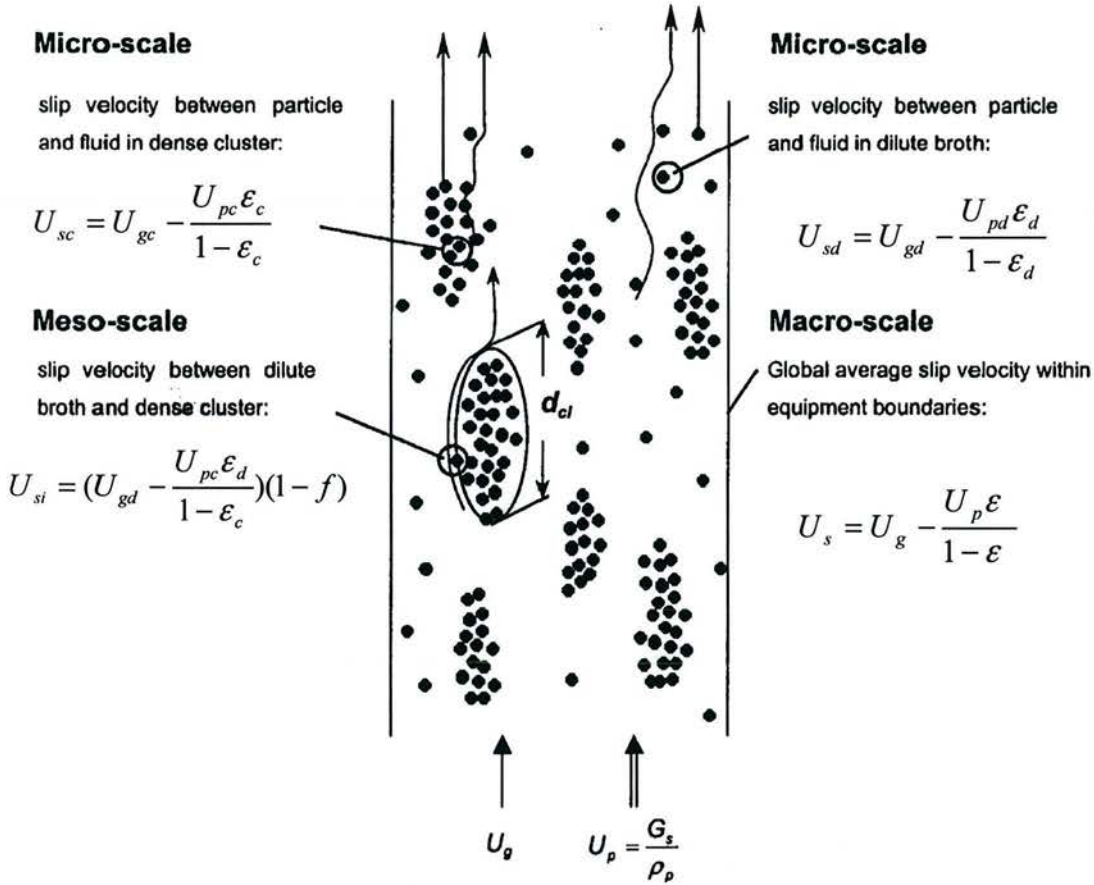
Fig.5-2 Three Scales of Interactions in Heterogeneous Gas/Solid Systems
