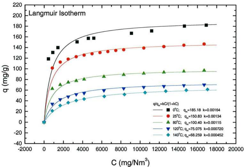
Fig. 2-7 Test Data Fitted With Langmuir Isotherm
