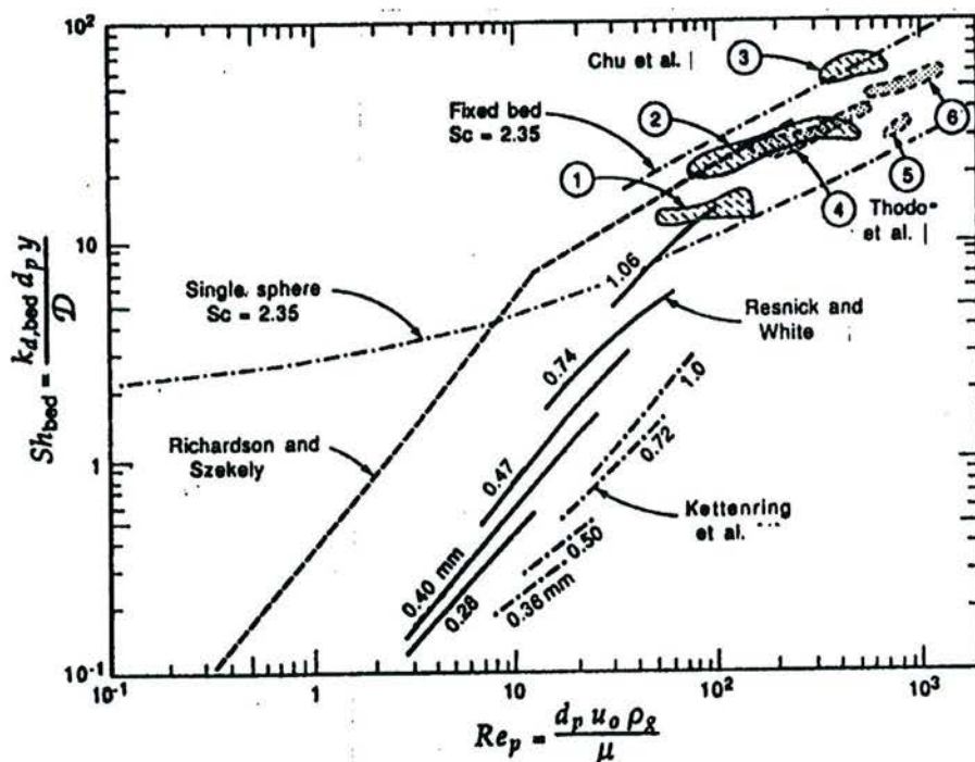
Fig. 6-1. Experimental Findings on Mass Transfer in Fluidized Beds (Kunii [55] )
