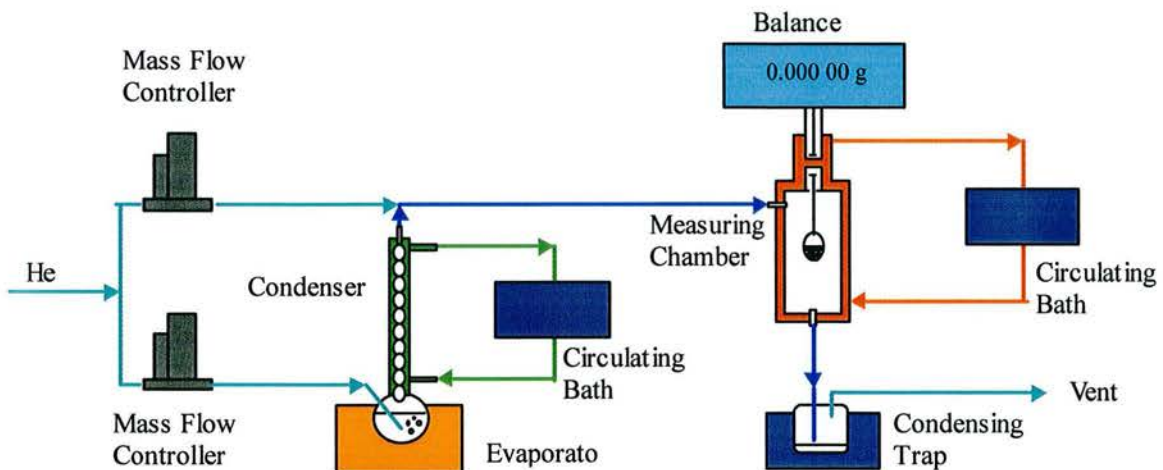
Fig. 2-2 Isotherm Measurement Setup
