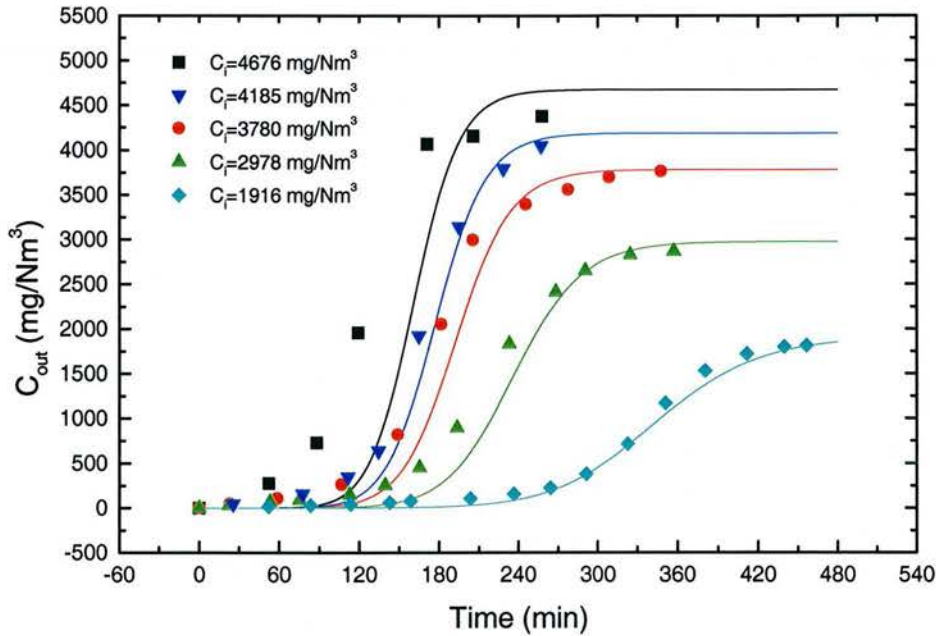
Fig. 4-2 Exit Gas Phase Concentrations with Different Inlet VOCs Concentrations
