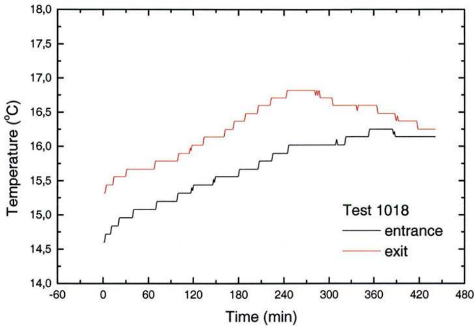
Fig. 3-7 Temperature History of Experiments
