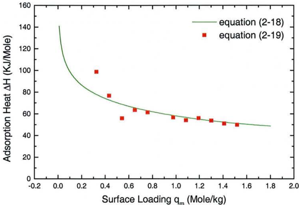
Fig. 2-12 Isosteric Heat vs Surface Loading
