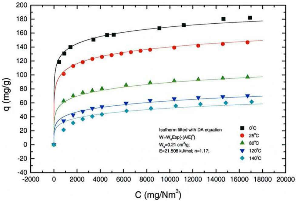
Fig. 2-11 Test Data Fitted with D-A Equation
