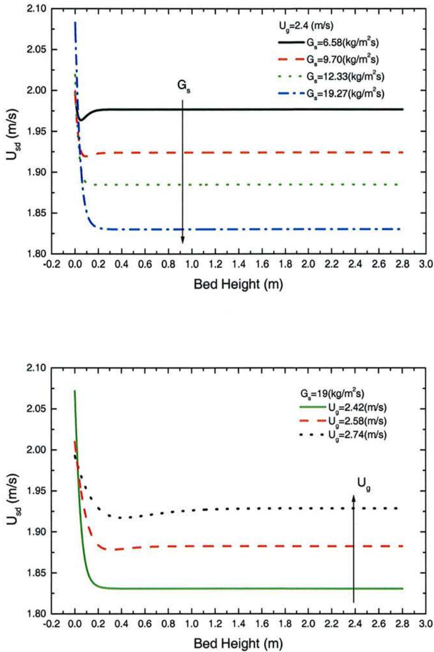
Fig. 5-18 U_{sd} Distribution Along CFB Riser at Different U_g and G_s
