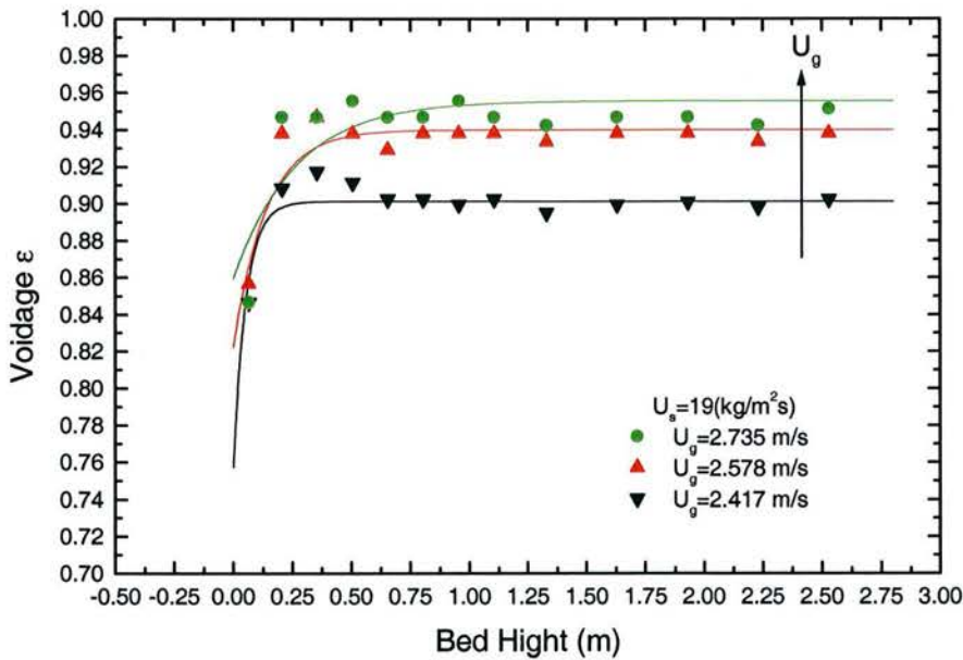
Fig. 5-15 Axial Voidage Distribution for Different G_s and U_g
