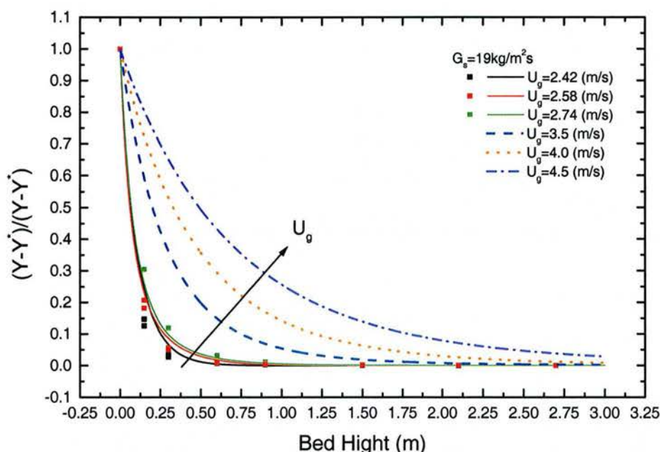
Fig. 7-4 Residual Concentration Distribution with Different Gas Velocities
