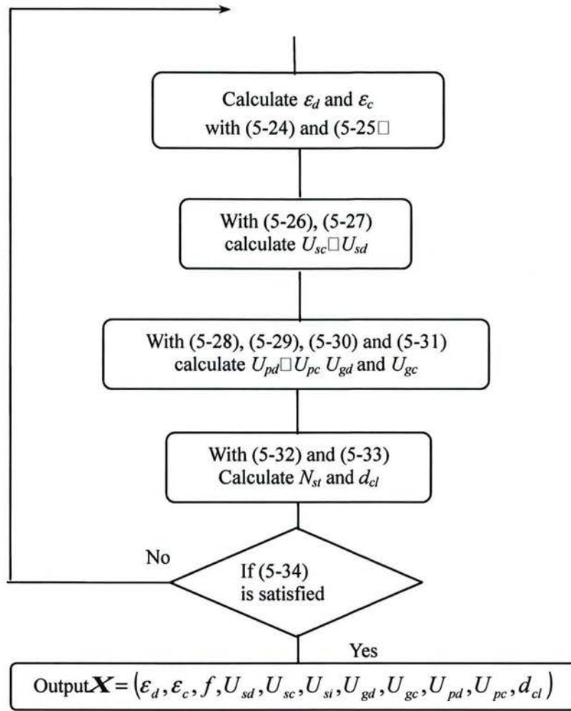
Fig. 5-3 Calculation Procedure of PFD Model.
