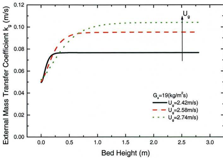
Fig. 6-5 The Changes of External Mass Transfer Coefficient along the Bed Height under Various Operating Conditions
