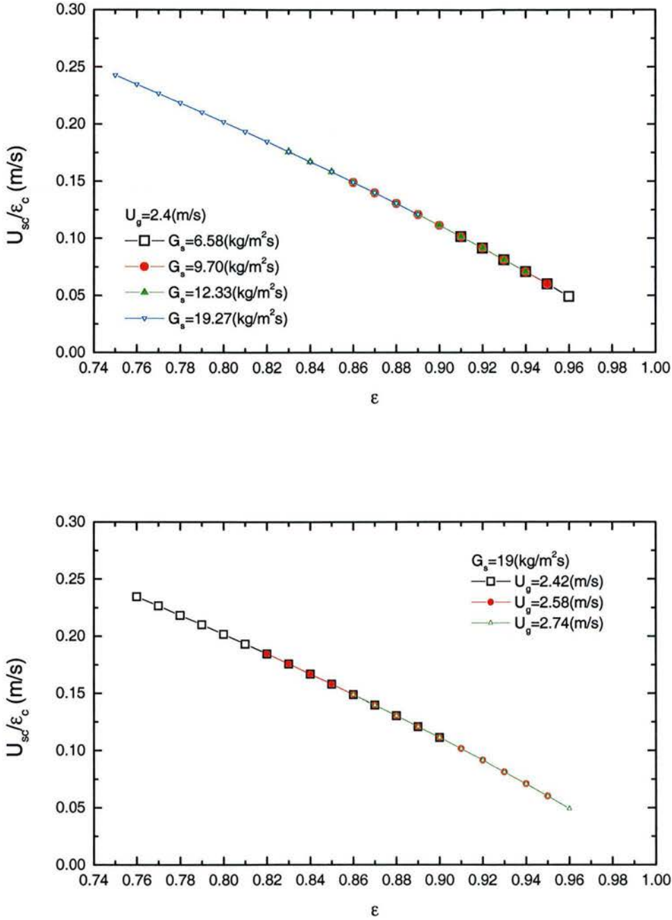
Fig. 5-10 Real Slip Velocity in the Cluster Phase at Different U_g and G_s
