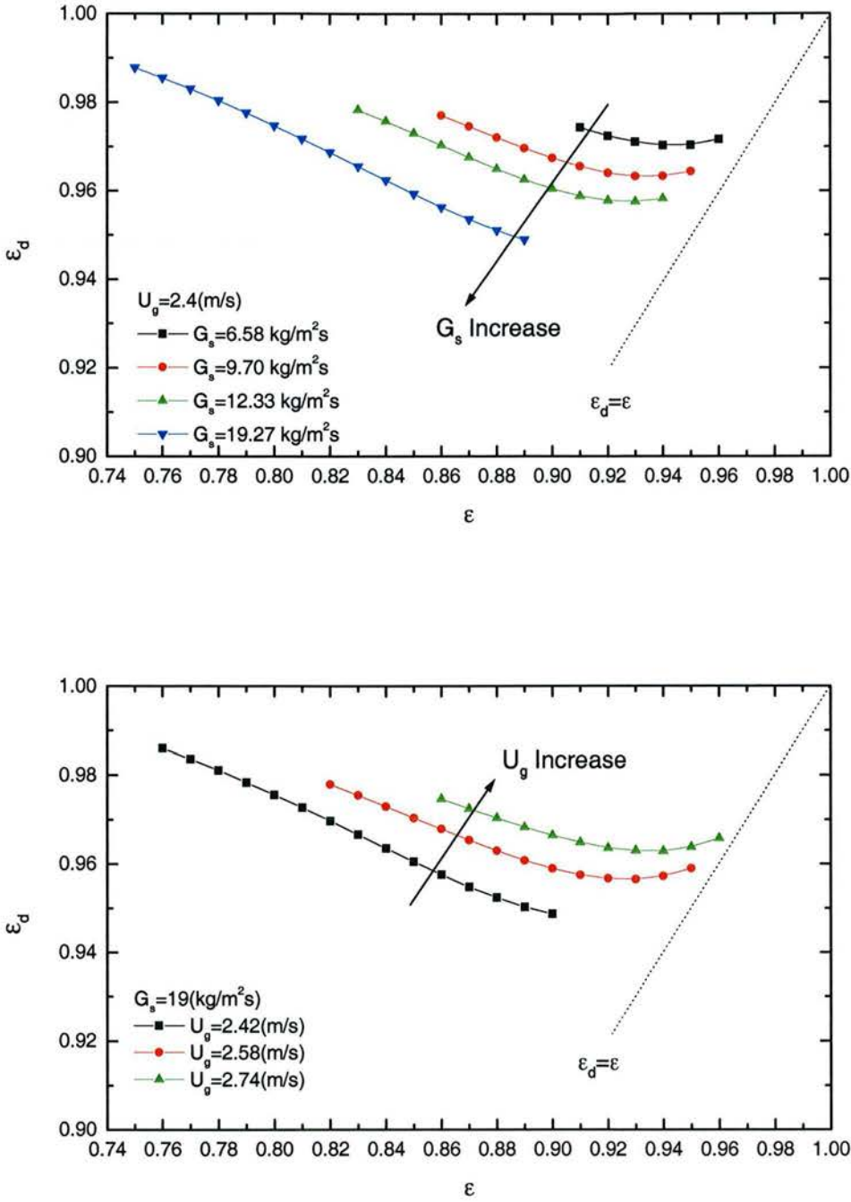
Fig. 5-4 Relation Between \epsilon_d and \epsilon at Different U_g and G_s
