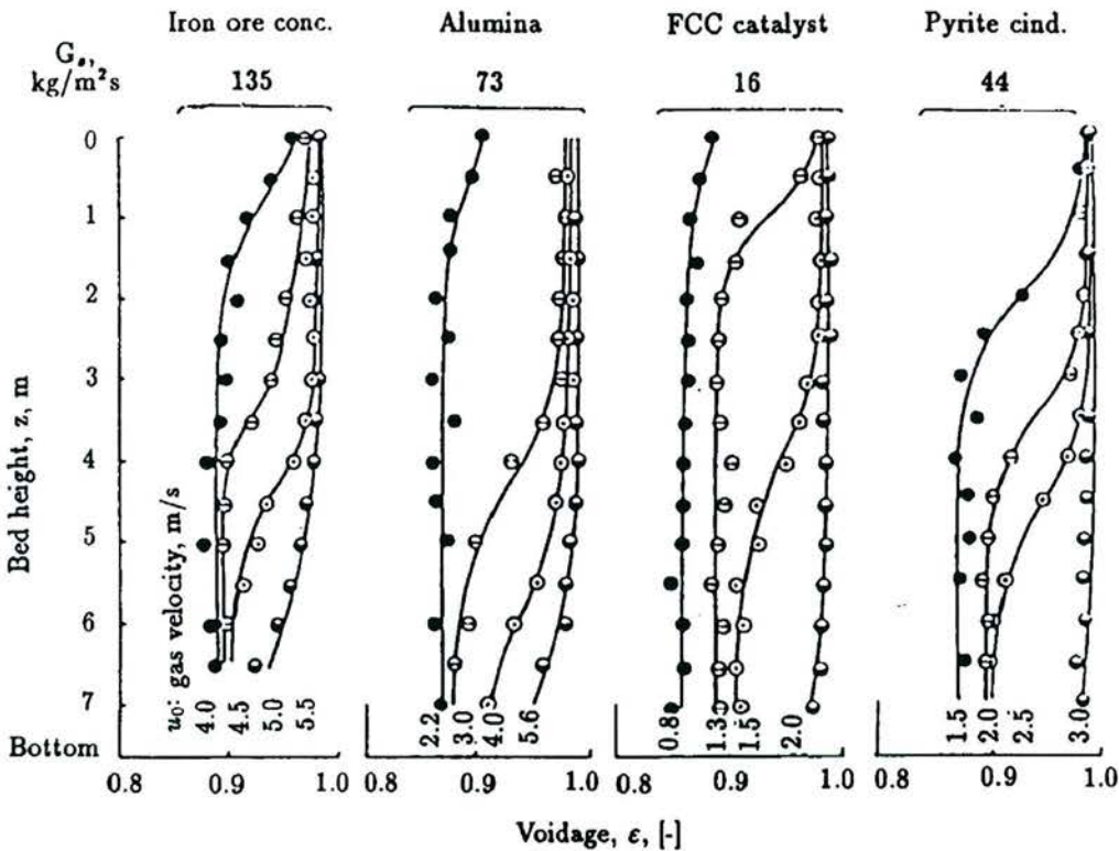
Fig. 5-14 Axial Voidage Distribution
