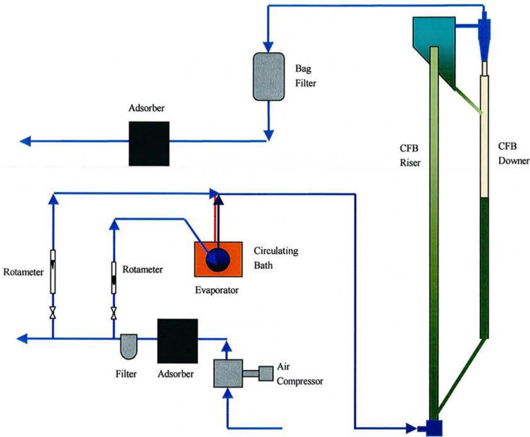
Fig. 3-1 Schematic Diagram of CFB Adsorption experimental setup
