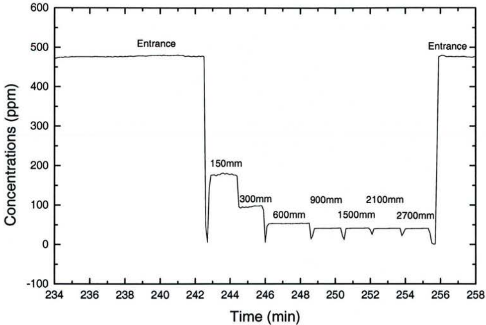
Fig. 3-6 Concentration Records of PGM-7600 During Experiment
