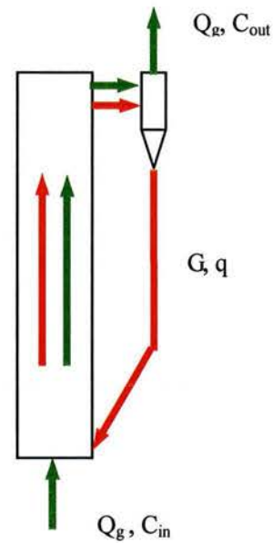
Fig. 4-1 CFB Adsorption System
