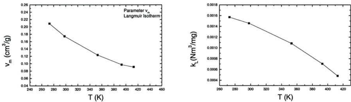
Fig. 2-6 Temperature Dependence of Langmuir Parameters v_m and k
