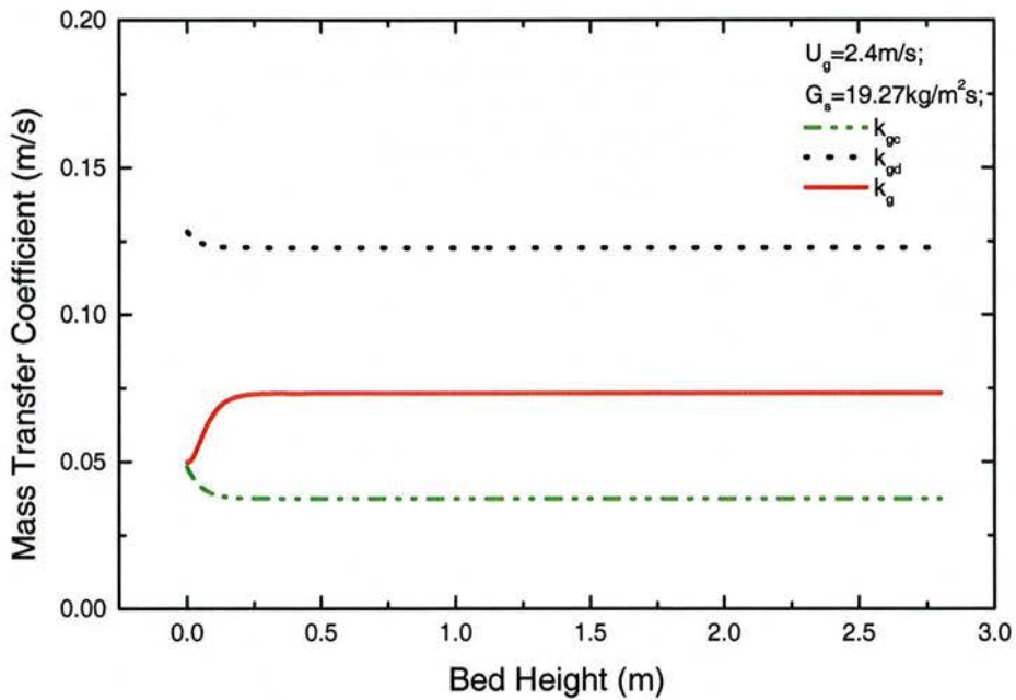
Fig. 6-4 External Mass Transfer Coefficient in the Bed
