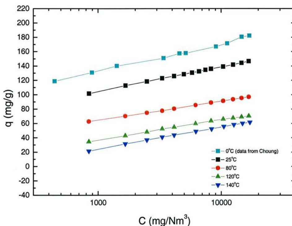
Fig. 2-3 Equilibrium Isotherm of Toluene/Ambersorb 600
