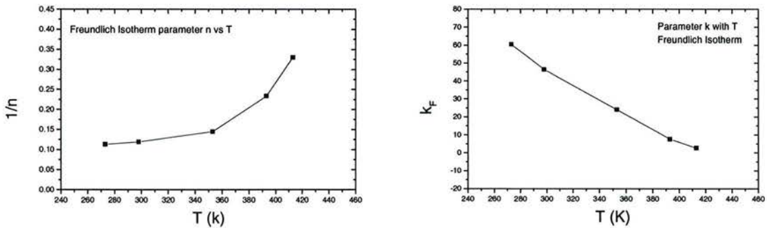
Fig. 2-10 Temperature Dependence of Freundlich Parameters 1/n and k
