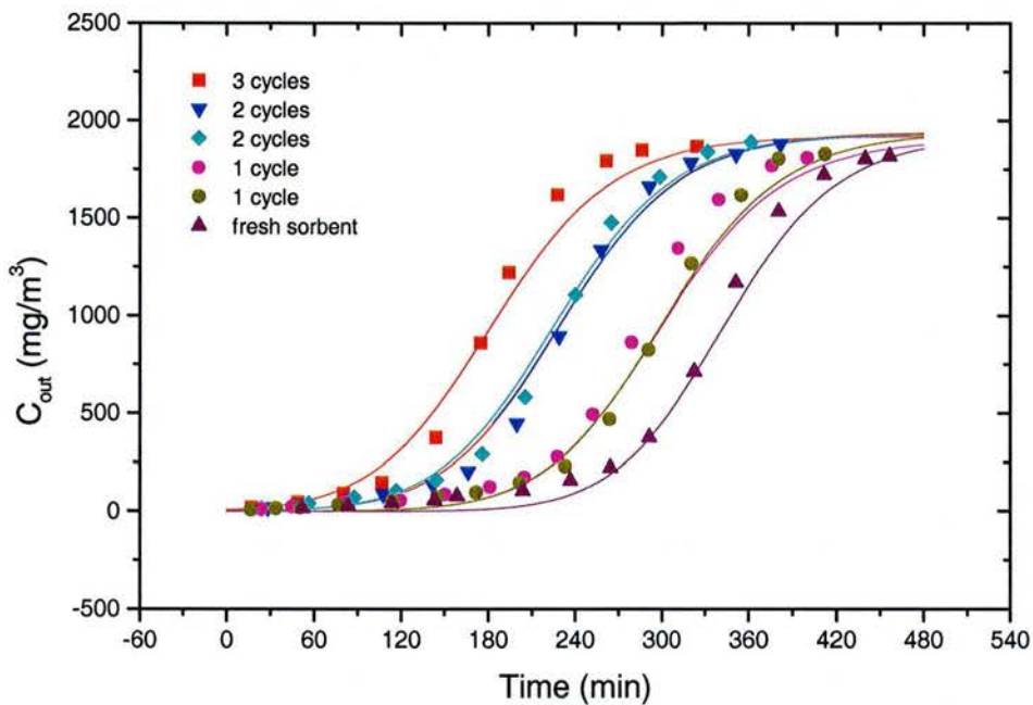
Fig. 4-5 Exit VOCs Concentrations with Different Fresh and Regenerated Adsorbent
