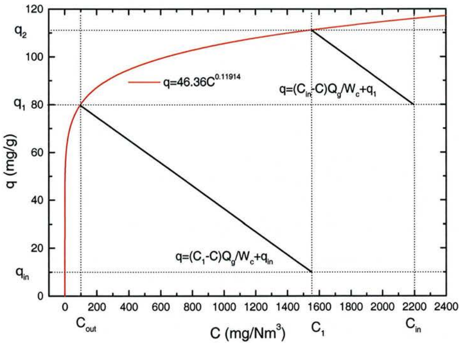
Fig. 7-9 Operation Lines in Two-stage CFB Adsorber
