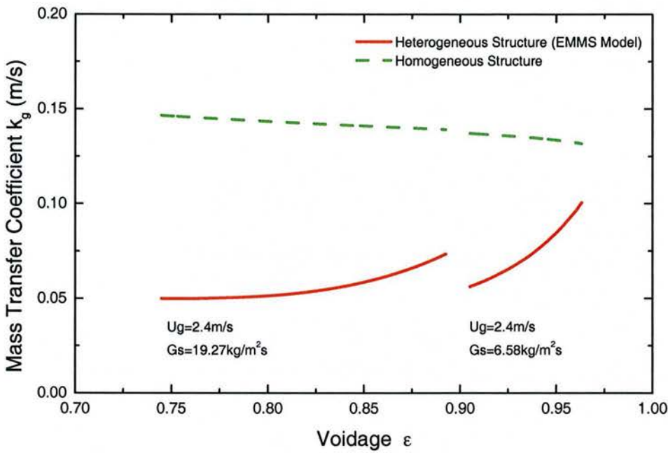
Fig. 6-3 Cross sectional averaged gas/solid mass transfer coefficient in CFB
