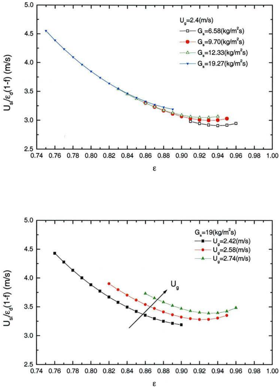
Fig. 5-13 Real Slip Velocity Between Dilute Gas and Clusters at Different U_g and G_s
