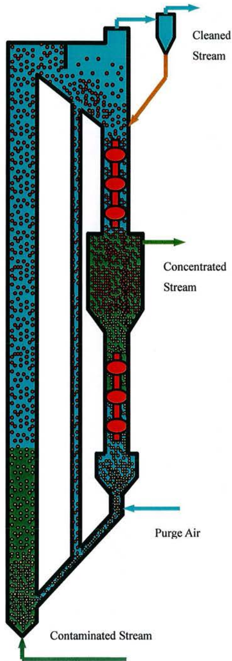
Fig. 7-10 CFB-PSA Process
