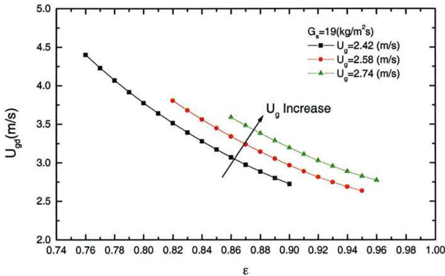
Fig. 5-5 Relation Between U_{gd} and \epsilon at Different U_g and G_s
