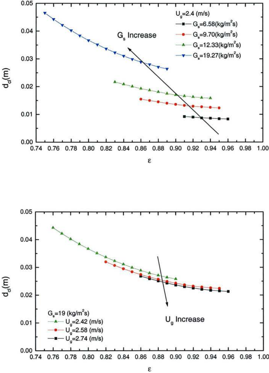
Fig. 5-12 Relation Between d_{cl} and \varepsilon at Different U_g and G_s
