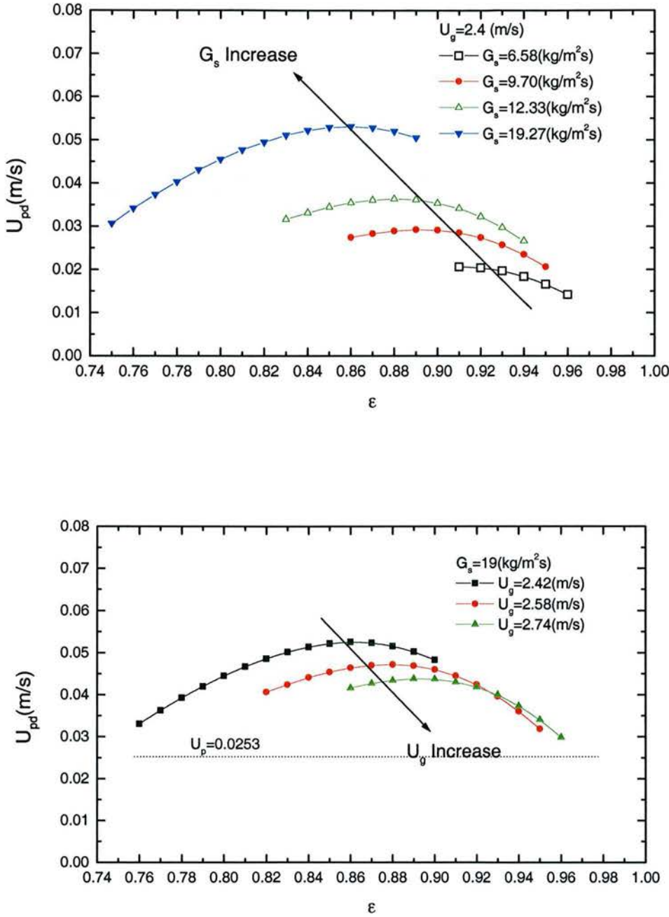
Fig. 5-6 Relation Between U_{pd} and \epsilon at Different U_g and G_s
