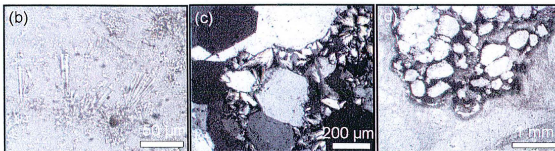
Figure 10 – (a) Mineral paragenesis established in the sandstone of the Maw Zone. The diagram represents successively sandstone deposition, diagenesis and a hydrothermal event of yttrium mineralization and uranium enrichment. Vertical lines represent fracturing and hydraulic brecciation events. The thickness of the black rectangles is representative of the abundance of the corresponding phase. (b), (c) and (d) Microscopic photographs. (b) Radiated needles of probably Cr-rich dravite originating from surface defects on a detrital quartz grain (polarized transmitted light). (c) Spherulitic aggregates of dravite surrounding corroded former euhedral quartz (plane polarized transmitted light). (d) Fragment of dravitized sandstone surrounded by euhedral quartz (polarized transmitted light).
