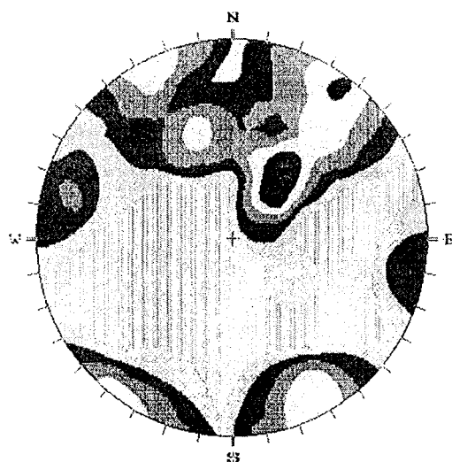
Figure 6 – Stereonet of the poles of the sandstone stratigraphy in the breccia fragments at the Maw Zone. Two main azimuths of tilting appear : N70 and N110.
