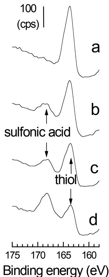
Fig. 4.7 . XPS spectra ( \text{S}_{2p} core-level) of MCM-41-SH after reaction with solutions containing Cr(VI) at increasing concentrations: (a) 50 \mu\text{M} , (b) 2 mM, (c) 5 mM and (d) 0.5 M.
