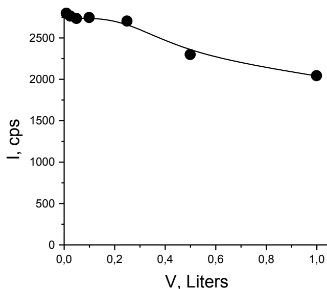
Fig. 5.11. Dependence of intensity of the chromium signal ( K\alpha line of Cr in XRF spectra) on Cr(VI) solution volume ( m_{\text{SiO}_2\text{-SH/ED3A}} = 100 \text{ mg} , n_{\text{Cr(VI)}} = 10 \mu\text{mole} , v = 1 \text{ mL min}^{-1} , \text{pH}=2,5 )
