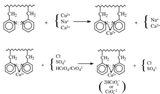
Fig. 1.9. Mechanism of simultaneous removal of heavy metal ions and chromates from a given medium.
