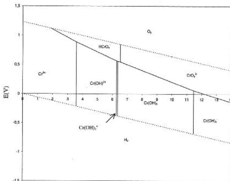
Fig. 1.2. A Pourbaix diagram for Cr species dominating in aerated aqueous solutions in the absence of any other complexing agents rather than OH - and H 2 O. Concentration of total chromium in solution is 10 -4 M. [3]
