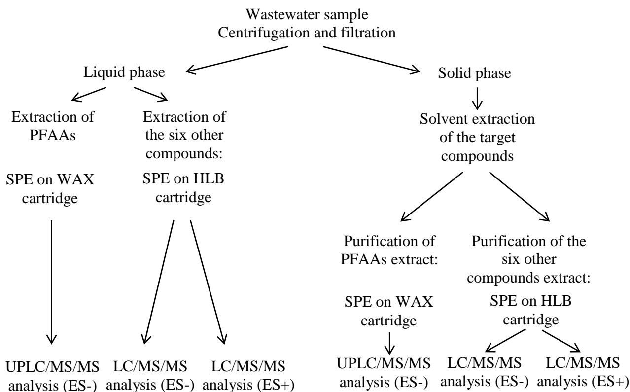
Figure 1. Schematic view of the extraction and analysis procedures of target compounds in wastewater and solid phases.
