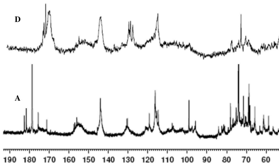
Fig.4. 7 ^{13}\text{C} -NMR spectra of grape pomace condensed tannins extracted by different extraction processes
