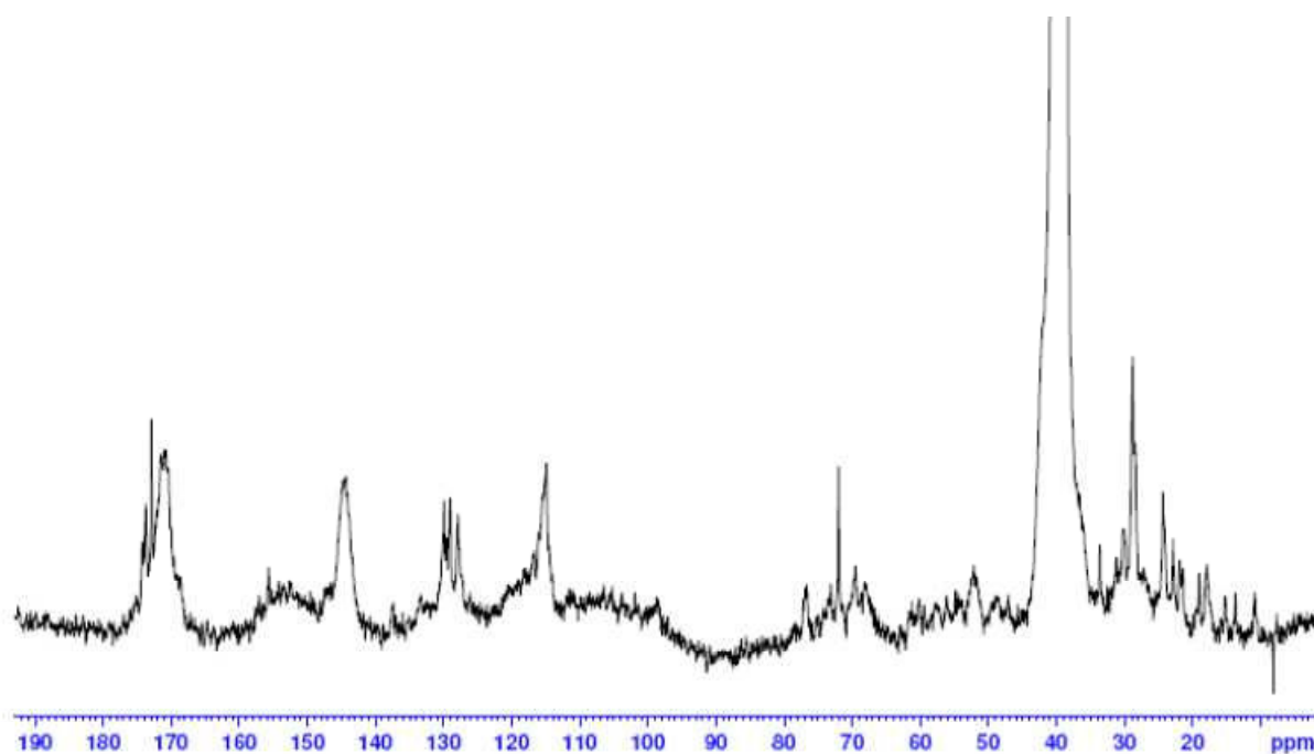
Annex 13. ^{13}\text{C} -NMR spectrum of acidified condensed tannins from grape pomace extracted by NaOH (5%)
