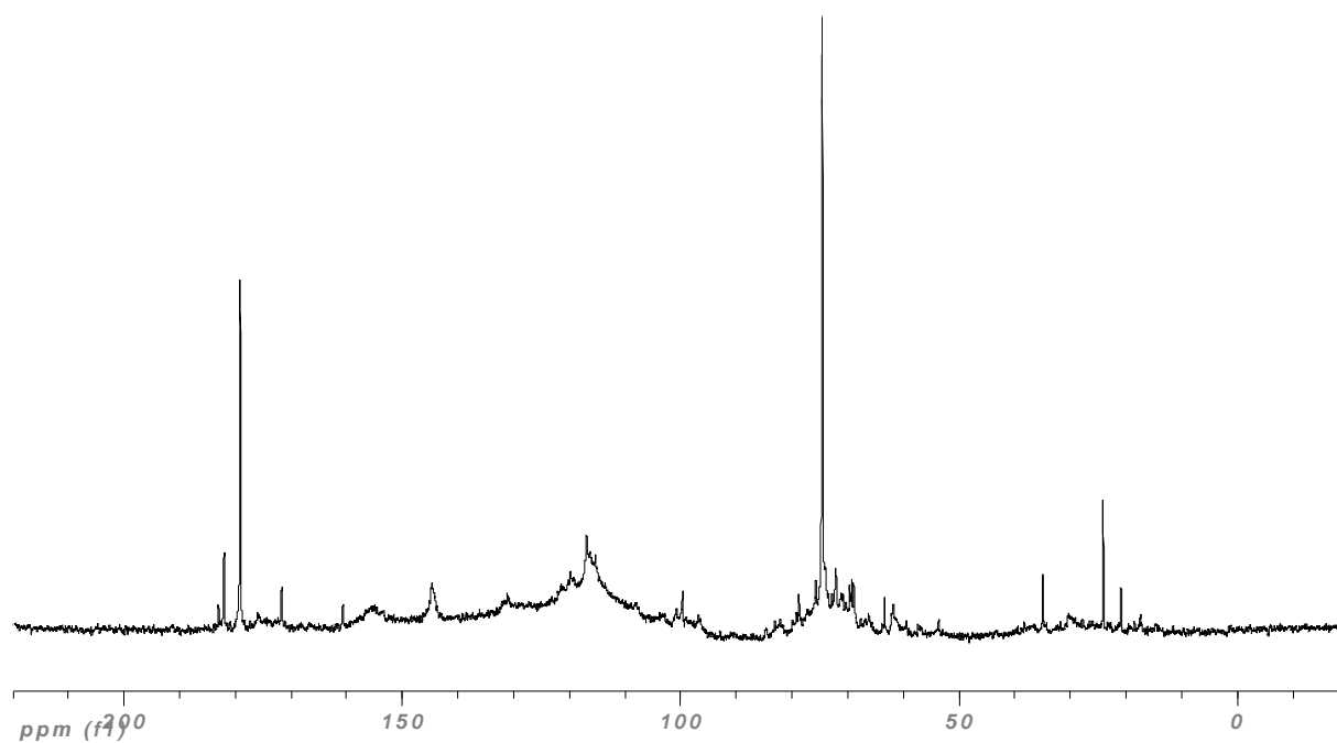
Annex 13. ^{13}\text{C} -NMR spectrum of acidified condensed tannins from grape pomace extracted by NaOH (5%)
