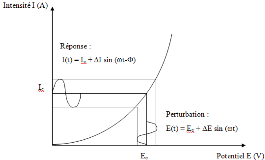
Figure 2.26 : Courbe I = f(E)
