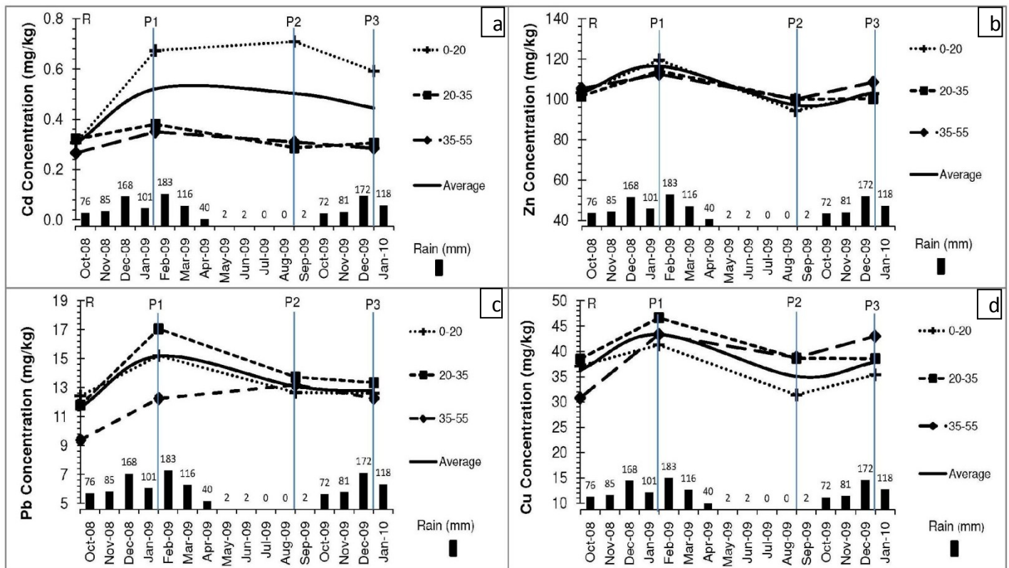
Figure 5. 2 Time-variation of TEs concentrations in the soil profile – Reference parcel R (T=0); PF-amended parcels P1 (T1 = 4 months); P2 (T2 = 11 months); and P3 (T3 = 15 months)
