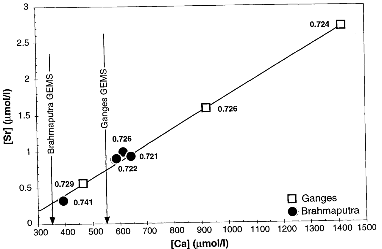
Fig. 10 : Ca versus Sr concentration relationship for Ganges (square) and Brahmaputra (circle) near their mouth. Data are from this study, Palmer and Edmond (1989); Sarin et al., (1989). ^{87}\text{Sr}/^{86}\text{Sr} values for each sample are indicated. During the monsoon, waters are more radiogenic and less concentrated. Based on this relationship and on the [Ca] yearly average given by the GEMS water program (arrows), average [Sr] for the Ganges and Brahmaputra should be 0.75 and 0.2 \mu\text{mol/l} respectively.
