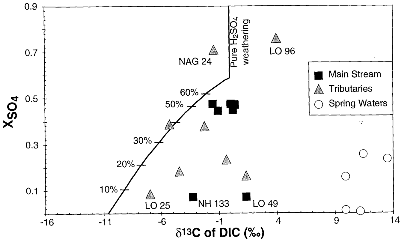
Fig. 6a : Plot of \delta^{13}\text{C}_{\text{DIC}} versus X\text{SO}_4 in the Kali Gandaki head waters. Data for thermal springs sampled near the river show high \delta^{13}\text{C} values, implying a metamorphic origin for the \text{CO}_2 . The mixing curve corresponds to the alteration by sulphuric acid and respired carbonic acid of 70% of carbonate and 30% of silicate. The fact that rivers plot to the right of the mixing curve implies that \text{CO}_2 rich in ^{13}\text{C} is involved in the alteration reaction in addition to biologic \text{CO}_2 . The contribution of metamorphic \text{CO}_2 dissolved in ground water as sampled in thermal springs is clearly identified at several locations.
