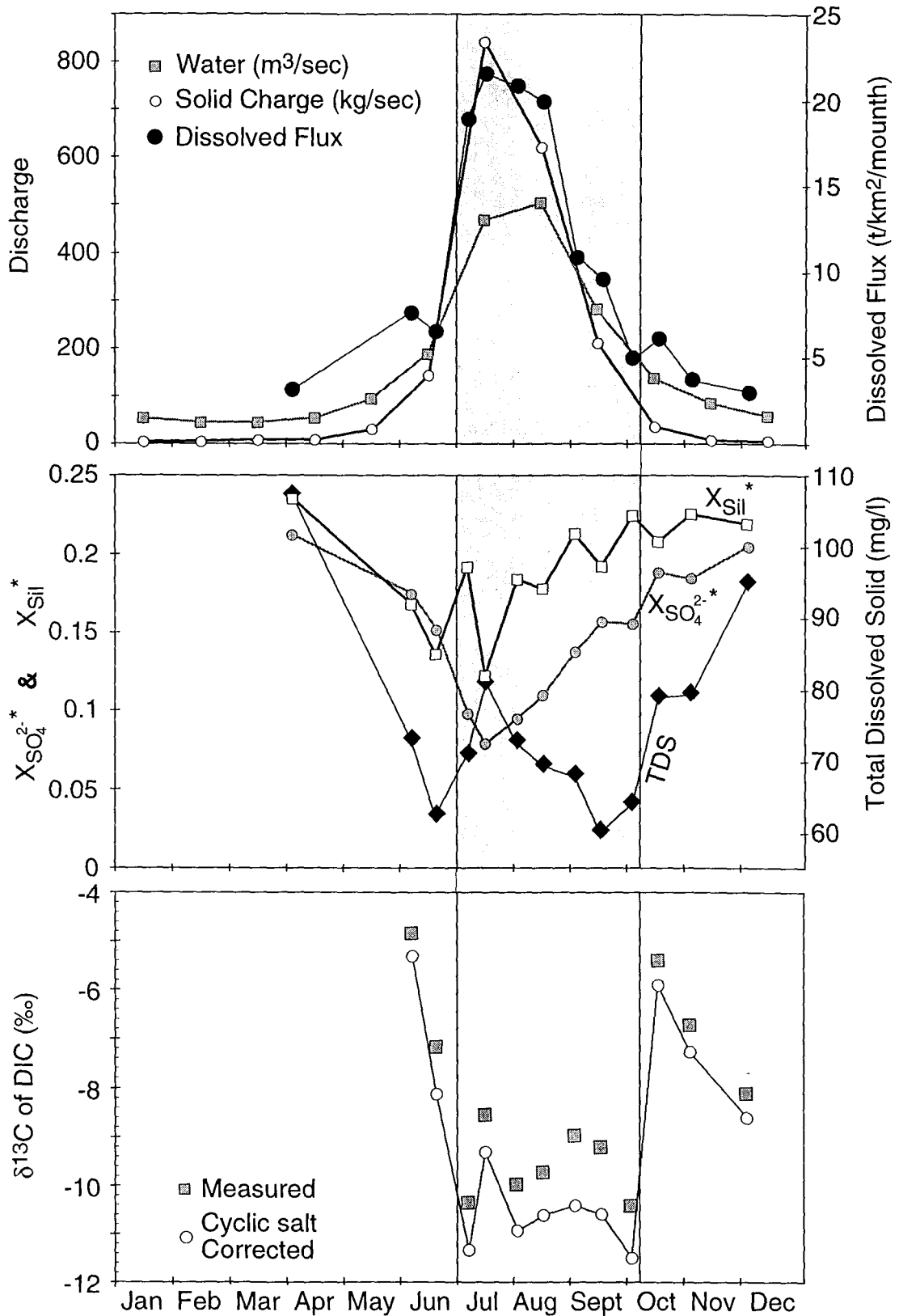
Fig. 7 : Seasonal variation of the water discharge and chemistry of the Trisuli river at Betrawati for TDS, X SO 4 2- *, X Sil * and δ 13 C DIC . The shaded area corresponds to the monsoon season. Water discharge data are from the Dept. of Hydrology and Meteorology of Nepal.
