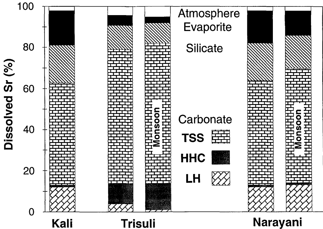
Fig 9 : Origin of Sr in term of lithologies for the Narayani and its two main tributaries. This budget derives from Sr isotopic mass balance (Fig. 8a) combined with lithological budget for each geological unit (Fig. 7).
