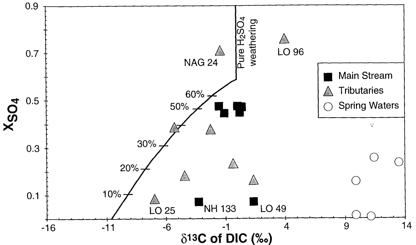
Fig. 6a : Plot of \delta^{13}C_{DIC} versus X_{SO_4} in the Kali Gandaki head waters. Data for thermal springs sampled near the river show high \delta^{13}C values, implying a metamorphic origin for the CO_2 . The mixing curve corresponds to the alteration by sulphuric acid and respired carbonic acid of 70% of carbonate and 30% of silicate. The fact that rivers plot to the right of the mixing curve implies that CO_2 rich in ^{13}C is involved in the alteration reaction in addition to biologic CO_2 . The contribution of metamorphic CO_2 dissolved in ground water as sampled in thermal springs is clearly identified at several locations.
