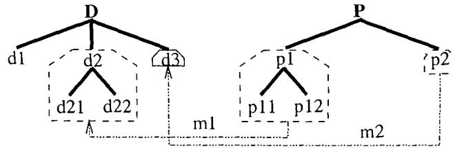
Figure 3.14: Versioning graph.
