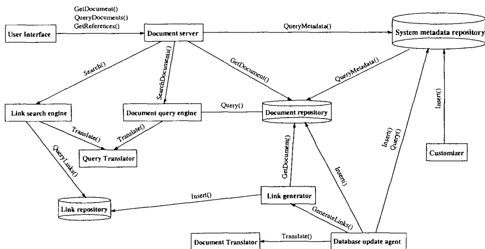
Figure 5.1: Components interaction.
