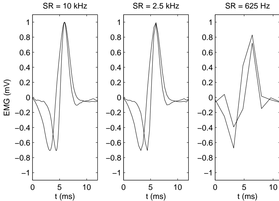
Figure 2.8: Two distinct action potentials recorded at 10 kHz are shown at left. The two following images show the same action potentials subsampled at 2.5 kHz and 625 Hz. The loss of information is clear in the last case.
