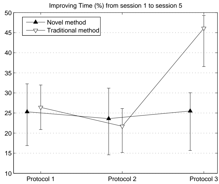
Figure 4.24: Learning for each protocol between the first and the last session. Error bars represent the 95% confidence interval.
