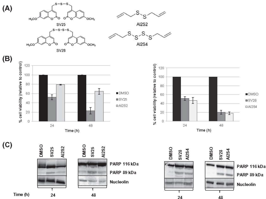
Figure 5. Coumarin polysulfides compared with diallyl polysulfides. (A) structures of two of the newly synthesised compounds—4,4'-disulfanedilylbis(methylene)bis(2 H -chromen-2-one) (SV25), and 4,4'-tetrasulfanedilylbis(methylene)bis(2 H -chromen-2-one) (SV28) with their corresponding well characterized diallyl polysulfides—diallyl disulfide (AI 2 S 2 ) and diallyl tetrasulfide (AI 2 S 4 ). (B), Cells were seeded in 24-well plates and treated with 0.05% DMSO as a control, 50 μM SV25 or 50 μM AI 2 S 2 for 24 h or 48 h. In a second set of experiments, cells were treated with 0.05% DMSO as a control, 50 μM SV28 or AI 2 S 4 for 24 h or 48 h. Afterwards, MTT assay was done to determine the number of viable cells in both set of experiments as in Figure 1B. Data are depicted as means ± SD, ( n = 3). (C), HCT116 cells were treated for 24 or 48 h with 0.05% DMSO as a control, 50 μM SV25 or AI 2 S 2 . In a second set of experiments, cells were treated with 0.05% DMSO as a control, 50 μM SV28 or AI 2 S 4 for the same time periods. (D) Cell extracts were treated for PARP cleavage as in Figure 3. Nucleolin was used as a loading control.
