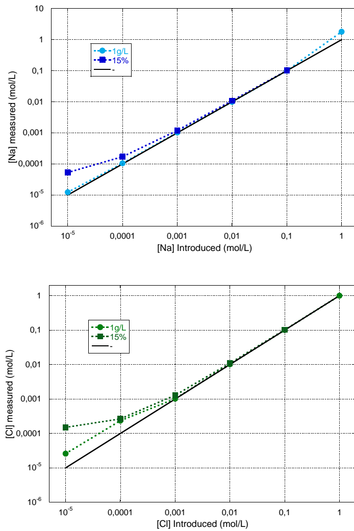
Figure 3.8 – Cl^- and Na^+ measured concentrations in 1 \text{ g}\cdot\text{L}^{-1} and 175 \text{ g}\cdot\text{L}^{-1} (i.e. 4,2% vol.) alumina slurries as a function of the concentrations introduced.
