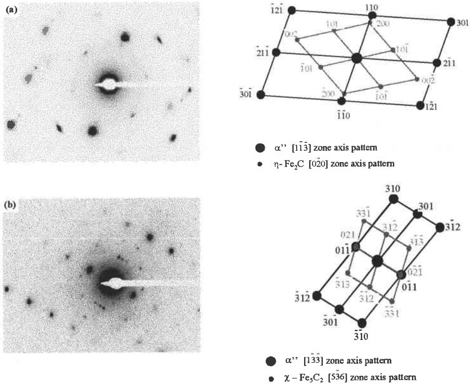
Figure 4 Diffraction patterns and their indexing of (a) \eta -Fe 2 C formed during non-magnetic tempering at 200°C for 60 min and (b) \chi -Fe 5 C 2 formed during magnetic tempering at 200°C for 60 min.
