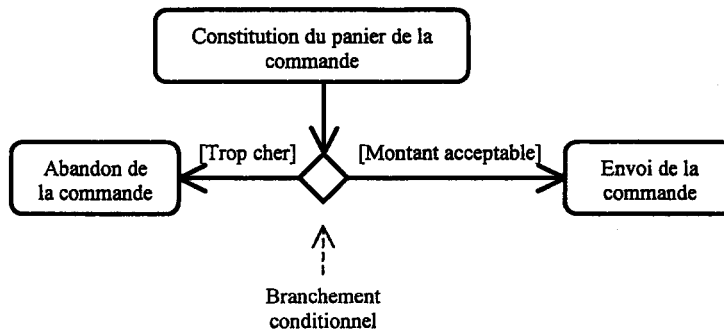
Figure 33 – Branchement conditionnel
