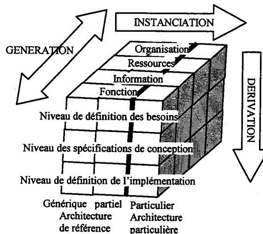
Figure II.5-1- Cube CIMOSA
