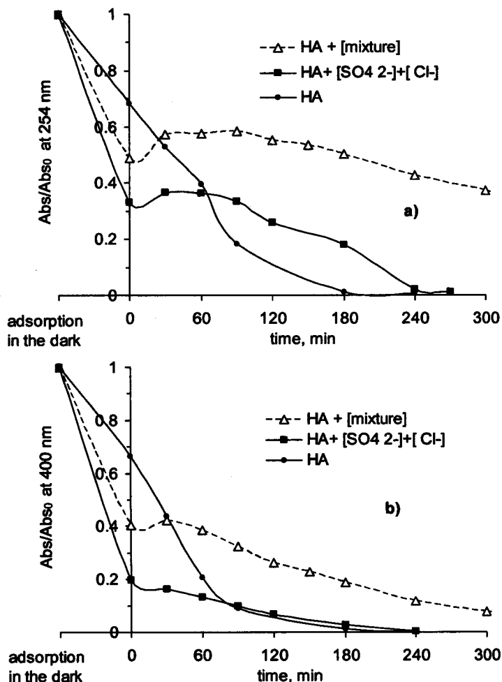
Figure 3.19 Effect of the mixture [ \text{Na}_2\text{SO}_4 , NaCl and \text{NaHCO}_3 ], so-called [mixture] and [ \text{Na}_2\text{SO}_4 and NaCl] on photodegradation of HAs a) Abs at 254 nm disappearance b) Colour removal (Abs at 400 nm)
