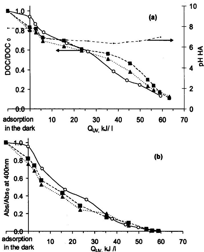
Figure 3.23 Effect of inorganic anions on a) mineralization and b) colour removal of HA solution versus accumulated UV energy. \text{TiO}_2 = 0.2 g/l; ( \circ ) HA; ( \triangle ) HA + [Cl^-] (4.5 g/l); ( \blacksquare ) HA + [SO_4^{2-}] (7.75 g/l) and (—) pH HA
