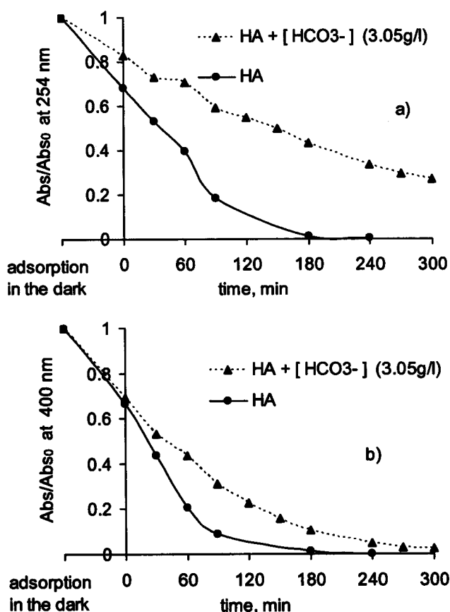
Figure 3.16 Influence of \text{NaHCO}_3 on photodegradation of HAs a) Abs at 254 nm disappearance b) Colour removal (Abs at 400 nm)
