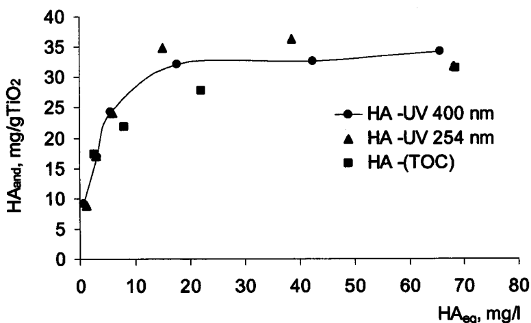
Figure 3.1 Adsorption isotherms of HAs (pH 7.8) on \text{TiO}_2
