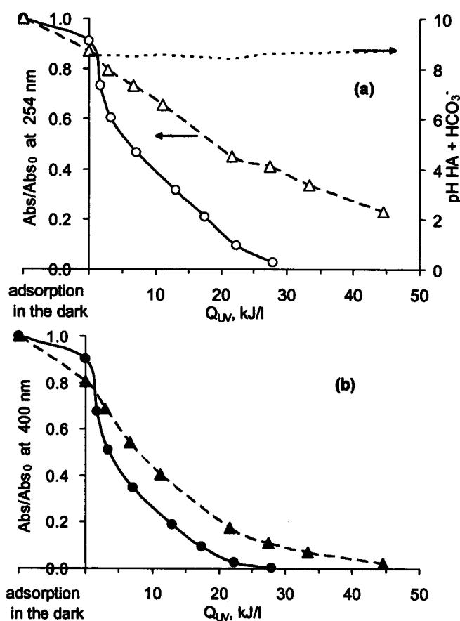
Figure 3.24 Effect of carbonate ions (3.05 g/l) on: a) absorbance at 254 nm and b) colour removal of HA solution versus accumulated UV energy, \text{TiO}_2 = 0.7 g/l. ( -\Delta- ) HA + [\text{HCO}_3^-] , ( -O- ) HA expressed as \text{Abs}/\text{Abs}_0 at 254 nm; ( -\blacktriangle- ) HA + [\text{HCO}_3^-] , ( -●- ) HA expressed as at \text{Abs}/\text{Abs}_0 at 400 nm and ( --- ) pH HA + [\text{HCO}_3^-]
