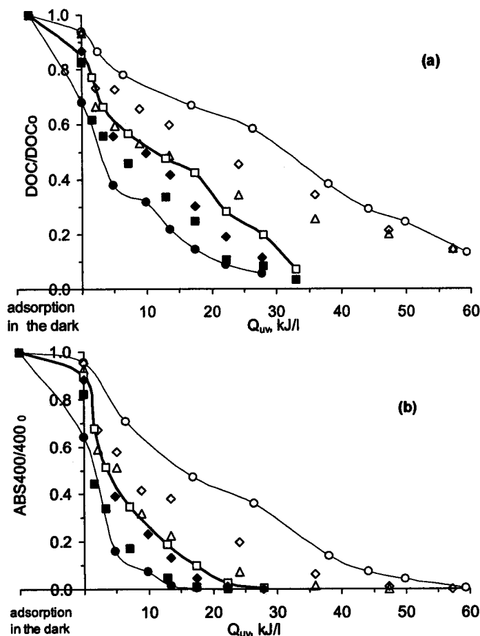
Figure 3.22 Influence of catalyst concentration on mineralization efficiency a) and b) colour removal of HAS solution versus accumulated UV energy. (○) \text{TiO}_2 = 0.2 g/l; (◇) \text{TiO}_2 = 0.3 g/l; (△) \text{TiO}_2 = 0.5 g/l; (□) \text{TiO}_2 = 0.7 g/l; (◆) \text{TiO}_2 = 1.0 g/l; (■) \text{TiO}_2 = 1.2 g/l; (●) \text{TiO}_2 = 2.0 g/l
