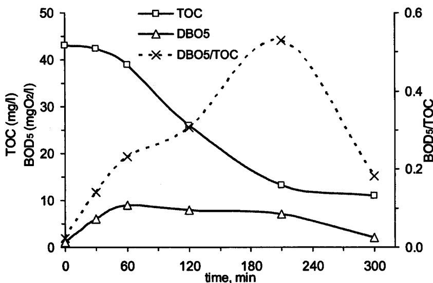
Figure 3.21 Evolution of \text{BOD}_5 and TOC during the irradiation of [\text{HA}] = 100 \text{ mg/l} with [\text{TiO}_2] = 1.0 \text{ g/l}
