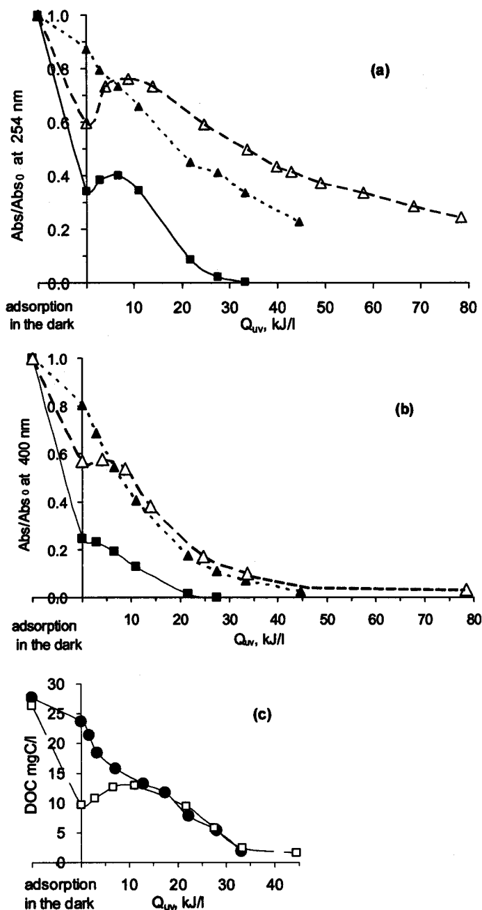
Fig. 3.25 Effect of mixture of inorganic anions in HA solution on a) Abs/Abs_0 at 254 nm, b) Abs/Abs_0 at 400 nm (colour) and c) DOC removal versus accumulated UV energy; \text{TiO}_2 = 0.7 \text{ g/l} ; (-\Delta-) HA + [HCO_3^- + Cl^- + SO_4^{2-}] ; (-\blacktriangle-) HA + [HCO_3^-] ; (-\blacksquare-) HA + [Cl^- + SO_4^{2-}] and (-\bullet-) DOC of HA; (-\square-) DOC of HA + [Cl^- + SO_4^{2-}]
