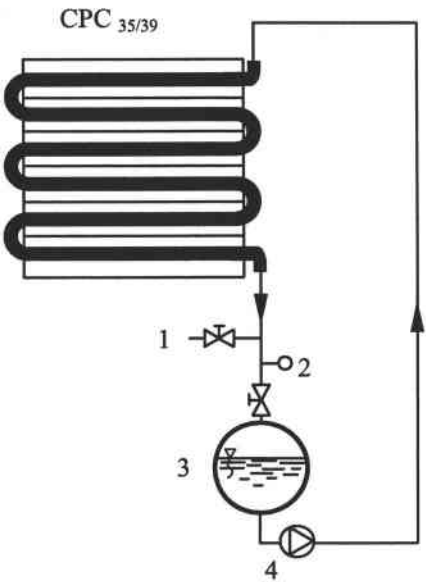
Figure 2.6 Picture of CPC 35/39 (left) and illustration-scheme of proceeding: 1-sampling valve, 2- thermocouple, 3- not-reacting tank, 4- pump (right)
