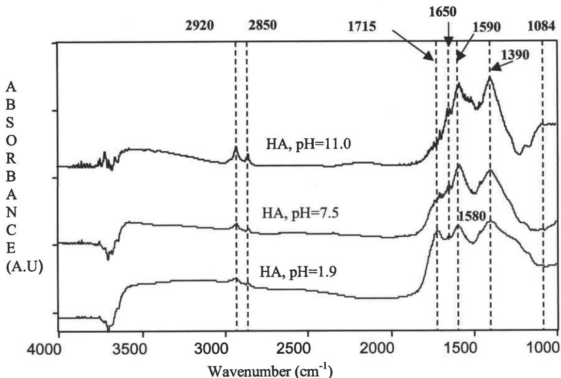
Figure 3.5 DRIFT spectrum of adsorbed HAs on \text{TiO}_2 at different pH
