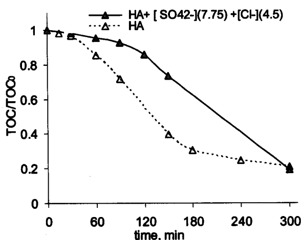
Figure 3.18 Influence of \text{Na}_2\text{SO}_4 and \text{NaCl} mixture on photomineralization (TOC) of HAs
