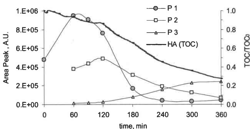
Figure 3.10 Evolution of Area Peak (P1-peak 1, P2-peak 2 and P3-peak 3) and TOC versus irradiation time during degradation of HAs
