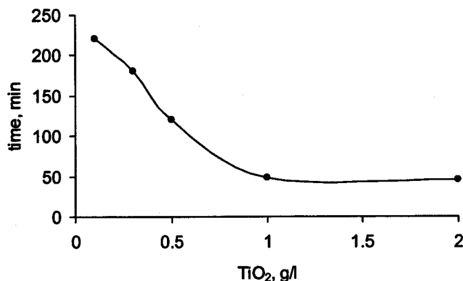
Figure 3.8 Evolution of the initial step (first domain) according to the \text{TiO}_2 amount
