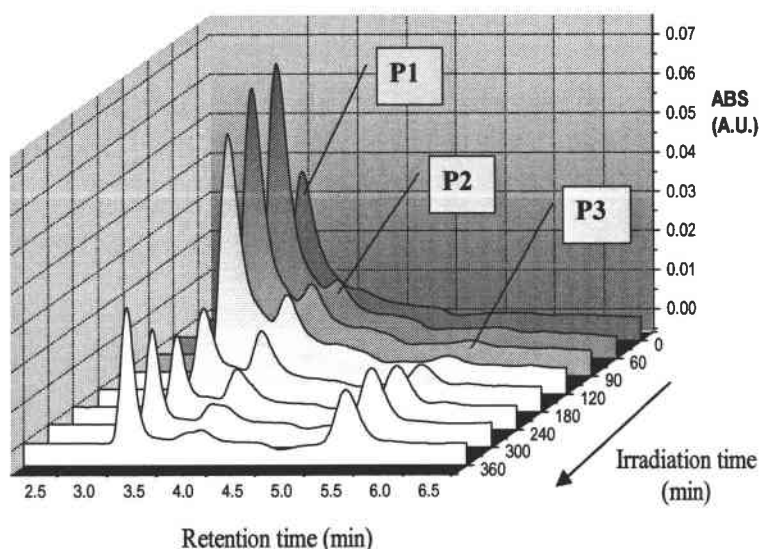
Figure 3.9 Chromatograms of photocatalytic degradation of humic acids intermediates with [\text{TiO}_2]=0.5\text{g/l}
