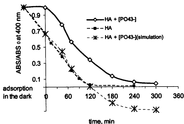
Figure 3.17 Effect of \text{Na}_2\text{HPO}_4 on colour removal of HAs
