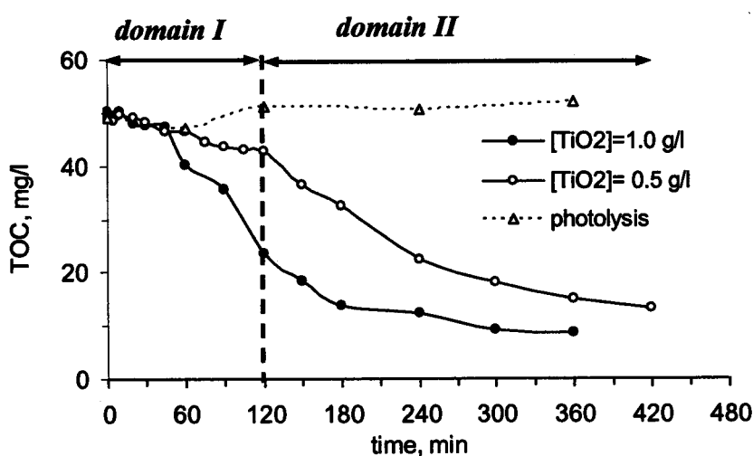
Figure 3.7 Photolysis and photomineralization of HAs equalling to 110 mg/l with [\text{TiO}_2] = 0.5 and 1.0 g/l
