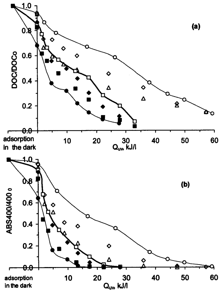
Figure 3.22 Influence of catalyst concentration on mineralization efficiency a) and b) colour removal of HAs solution versus accumulated UV energy. (○) TiO 2 =0.2 g/l; (◇) TiO 2 =0.3 g/l; (△) TiO 2 =0.5 g/l; (□) TiO 2 =0.7 g/l; (◆) TiO 2 =1.0 g/l; (■) TiO 2 =1.2 g/l; (●) TiO 2 =2.0 g/l
