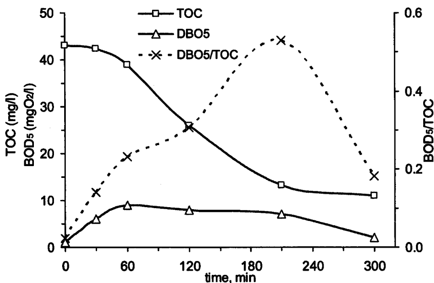
Figure 3.21 Evolution of \text{BOD}_5 and TOC during the irradiation of [\text{HA}] = 100 \text{ mg/l} with [\text{TiO}_2] = 1.0 \text{ g/l}
