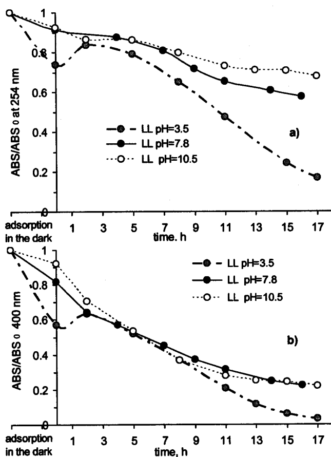
Figure 5.1 Effect of pH on photocatalytic degradation of landfill leachate amounting to COD= 210 mgO 2 /l, determined by a) normalised absorption at 254 nm and b) normalised adsorption at 400 nm (colour) evolutions
