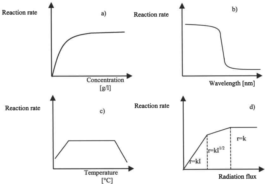
Figure 1.9. Influence of different parameters on photodegradation rate. a) catalyst dose and initial concentration of substrate, b) wavelength, c) temperature, c) radiation flux
