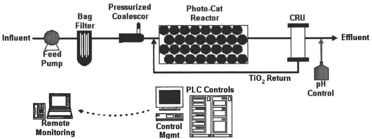
Figure 1.15 Scheme of the Photo-Cat® Water Treatment Train
