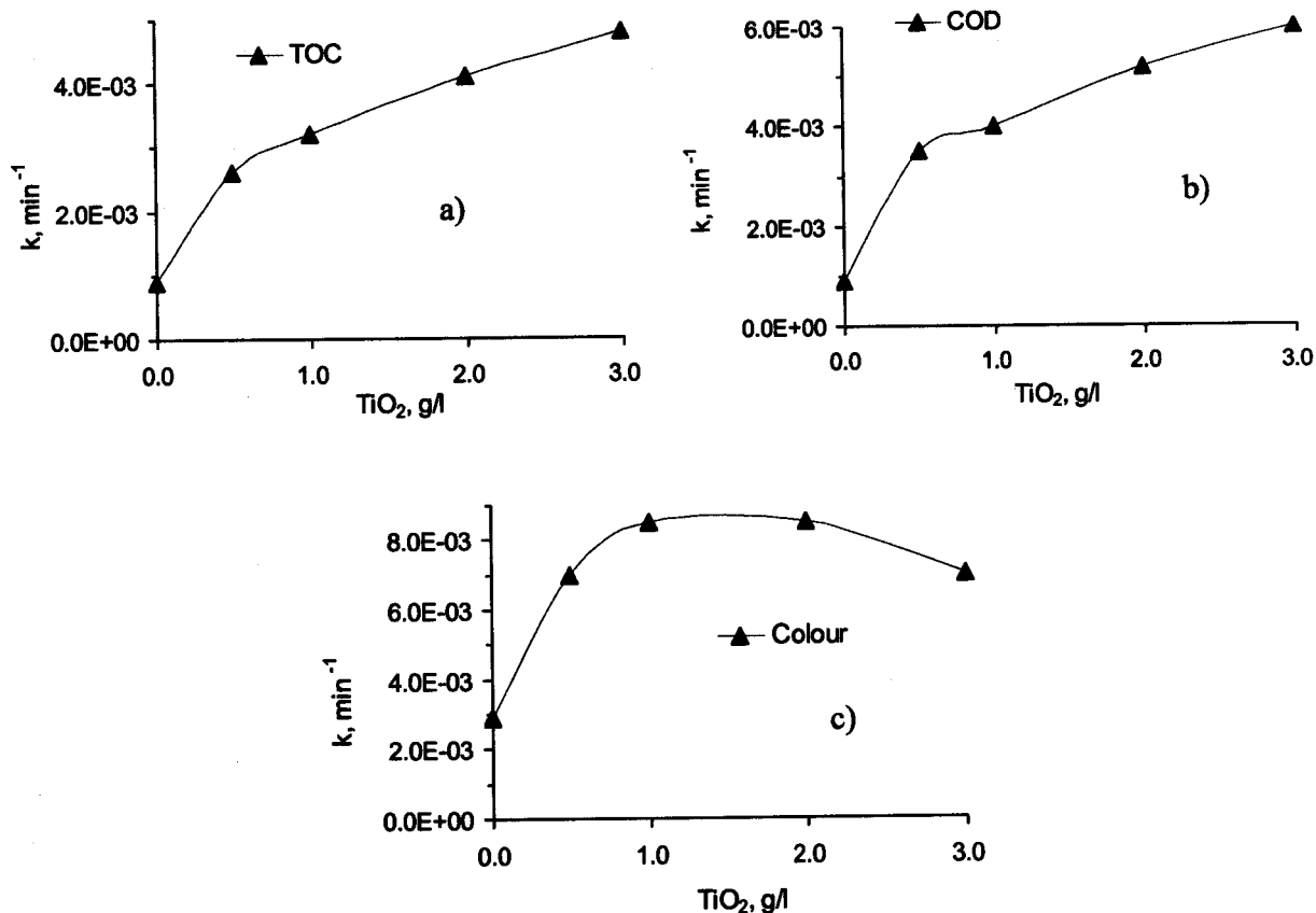
Figure 5.7 Effect of the photocatalyst (TiO 2 , P-25) concentration on the photodegradation rate of landfill leachate at pH 4; determined by a) TOC, b) COD and c) Colour
