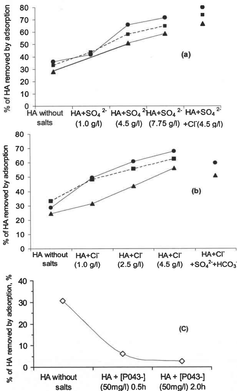
Fig. 3.6 Influence of ionic strength on affinity of HAs amounting to 100 mg/l to the catalyst surface. TiO 2 = 1.0 g/l and pH 7.5 (except the solution of HCO 3 - )
