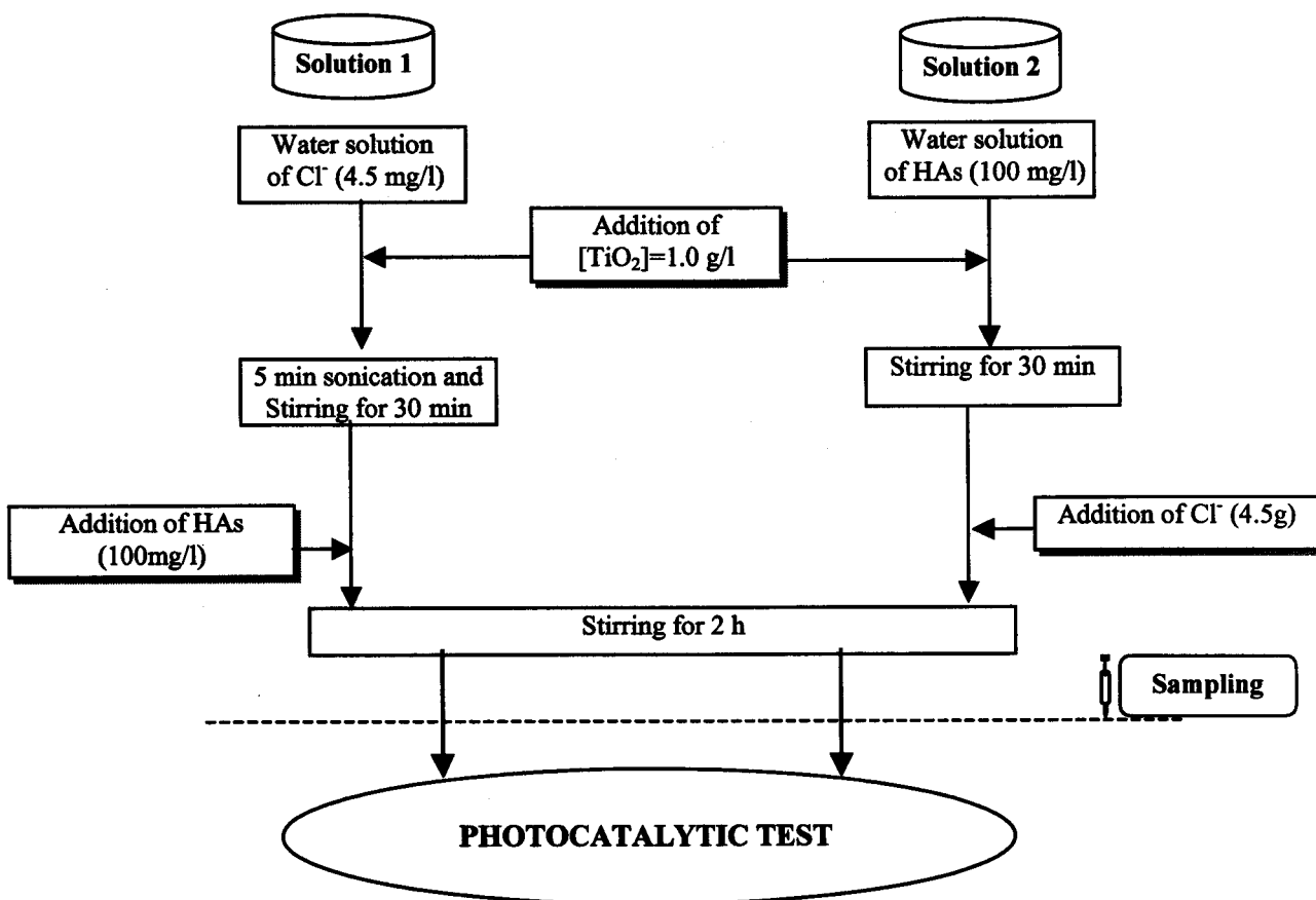
Figure 2.5 Procedures for the evaluation of \text{Cl}^- effect
