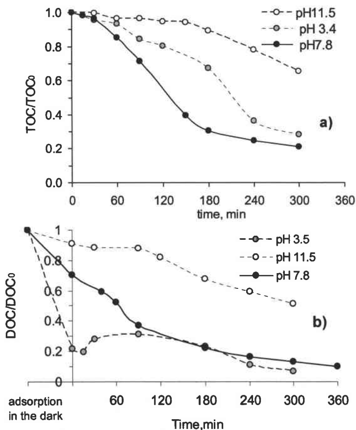
Figure 3.12 Evolution of a) TOC and b) DOC during illumination of humic acids solution ( [\text{HA}] = 100 \text{ mg/l} ) containing \text{TiO}_2 = 1.0 \text{ g/l} at different initial pH values (3.4, 7.8 and 11.5)
