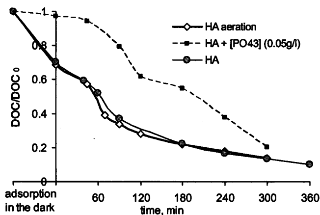
Figure 3.20 Effect of Na 2 HPO 4 and air-flow on photomineralization of HAs
