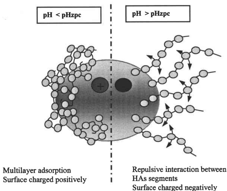
Figure 3.3 Model HAs adsorption on TiO 2 according to pH
