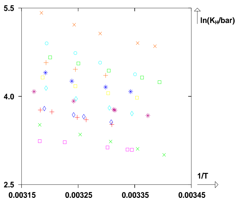
Figure IV-3: Henry's law constant of N 2 O in [P 14,666 ][Tf 2 N]( \times ), [N 6,111 ][Tf 2 N]( + ), [1-methoxyethanemim][Tf 2 N]( \diamond ), [1-ethanolmim][Tf 2 N]( * ), [emim][Tf 2 N]( \diamond ), [bmim][octysulfate]( \square ), [bmim][TfO]( * ), [bmim][BF 4 ]( + ), [bmim][beti]( \square ), [1-ethanolmim][PF 6 ]( \square ), [bmpy][BF 4 ]( \circ ) and [1-ethanolmim][BF 4 ]( \times ).
