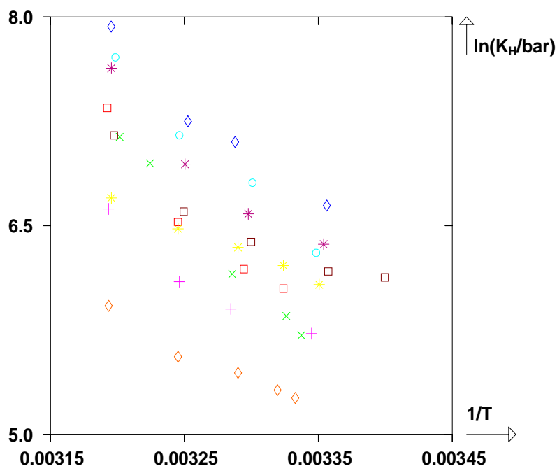
Figure IV-4: Henry's law constant of \text{CH}_4 in [1-ethanolmim][Tf 2 N](◇), [N 6,111 ][Tf 2 N](+), [emim][Tf 2 N](×), [bmim][octylsulfate](□), [bmim][CF 3 SO 3 ](□), [bmim][BF 4 ](◇), [1-ethanolmim][PF 6 ](*), [1-ethanolmim][BF 4 ](○) and [dmim][MePO 3 ](*).
