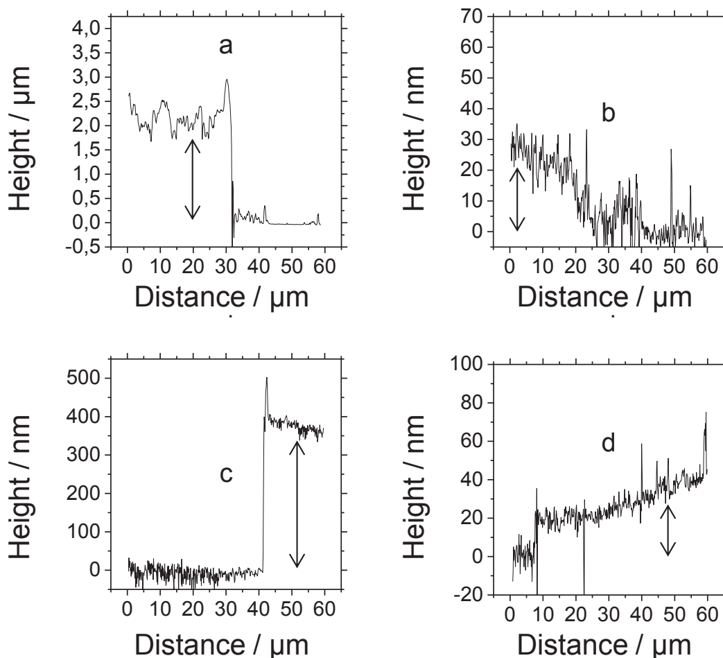
Fig II-1. AFM profiles measured on films composed with (a) TMOS, PEG, and chitosan, (b) TMOS and PEG, (c) TMOS and chitosan, (d) chitosan and PEG. N.B. E = -1.3\text{ V} , deposition time = 30s.
