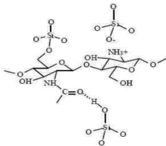
Fig I-5. Possible interactions between chitosan and silicates (adapted from reference [57]).
