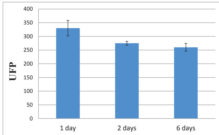
Fig V-3. Assessment of bacteriophage \Phi X174 infectivity along 6 days of dispersion in saturated solution of sodium silicate.
