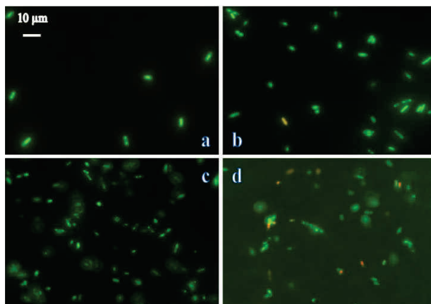
Fig II-12. Short-term BacLight analysis of EABE(1S) for E. coli C600 ( 4 \times 10^8 cells mL -1 ) along deposition times of optimal sol-gel: a) 10 s; b) 20 s; c) 30 s and d) 60 s. Same magnification for all pictures. All films have been prepared by electrolysis at -1.3 V with final cell density 10^8 cells/mL.
