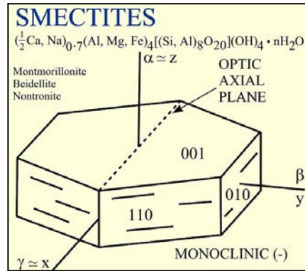
Figure 6 Smectites structure 241
