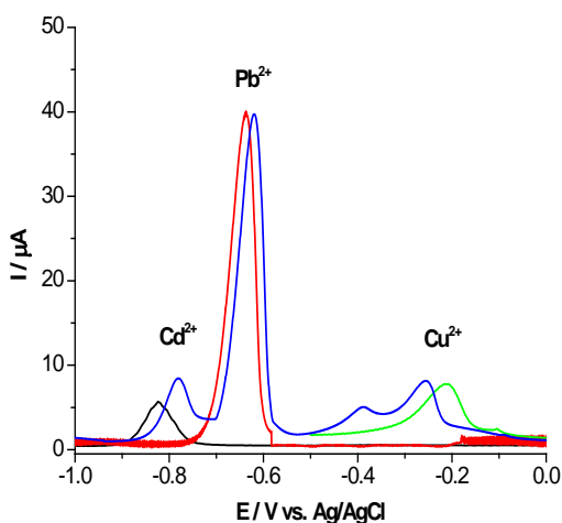
Figure 29 SWVs recorded using GCE+MMT+TBAB(-TBAB)/M, after 5 min accumulation at open-circuit in 10^{-5} M: \text{Cd}^{2+} (black), \text{Pb}^{2+} (red), \text{Cu}^{2+} (green) and a mixture of these three cations (blue) solutions in ultrapure water. Detection performed in 0.1M \text{NaNO}_3 solution, after 180 s electrolysis at -1.1 V (frequency: 100 Hz; amplitude: 0.05 V; potential step: 0.02; counter electrode: Pt/Ti; reference electrode: Ag/AgCl without internal solution).
