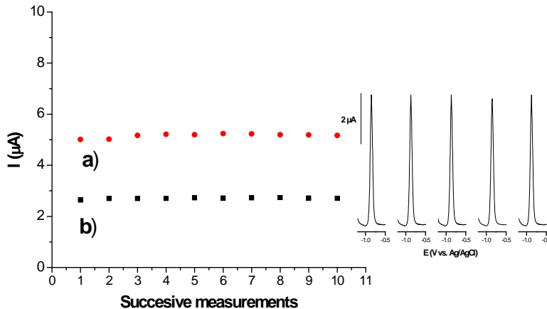
Figure 26 SWV responses obtained with (a) GCE+MMT/M and (b) GCE+MMT+TBAB(-TBAB)/M to successive preconcentration of 10^{-6} M \text{Cd}^{2+} solution (5 min accumulation at open circuit, detection in 0.1 M \text{NaNO}_3 after 180 s electrolysis at -0.6 V, regeneration after 120 s magnetic stirring in 0.1M \text{NaNO}_3 solution). The inset shows SWVs obtained using GCE+MMT+TBAB(-TBAB)/M after preconcentration in \text{Cd}^{2+} solution.
