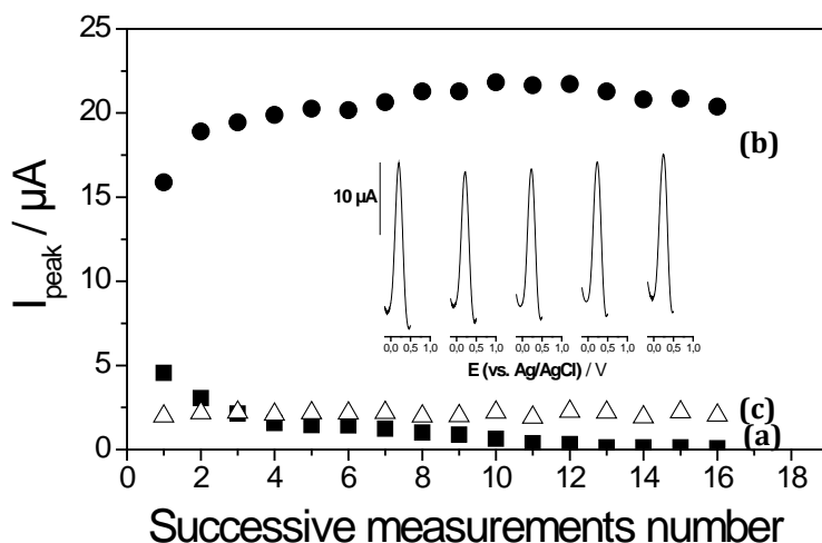
Figure 36 SWV responses obtained with (a) GCE-clay, (b) GCE-clay-mesopSiO 2 after surfactant removal, and (c) GCE-mesopSiO 2 , to successive pre-concentration of 10 -6 M Cu 2+ (2 min accumulation at open circuit; detection in 0.1 M KCl + 0.1 mM HCl). The inset shows some typical curves obtained with GCE-clay-mesopSiO 2 after surfactant removal (corresponding to data in part “b” of the figure).
