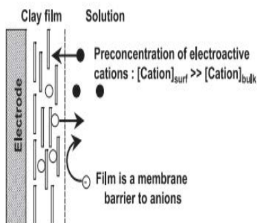
Figure 2 Preconcentration step at clay-modified electrode 2
