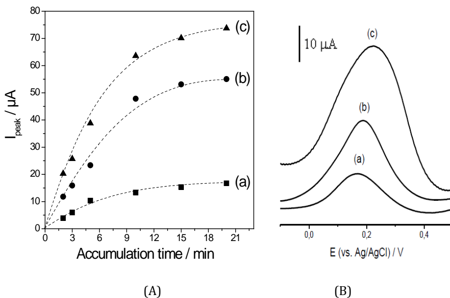
Figure 35 (A) Variation of SWV peak currents recorded using GCE-clay-mesopSiO 2 after open circuit accumulation of Cu 2+ at various concentrations: (a) 10 -7 M, (b) 5·10 -7 M, and (c) 10 -6 M. Detection medium composition: 0.1 M KCl + 0.1 mM HCl. (B) Typical SWV curves obtained at the above different concentrations of Cu 2+ but at the same preconcentration time (5 min).
