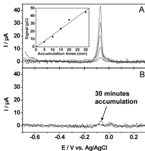
Figure 5 Influence of the pre-concentration time on the voltammetric response of carbon paste electrodes modified with (A) a mercaptopropyl-functionalized mesoporous silica prepared from a TEOS/MPTMS 80 : 20 and (B) an amorphous silica gel grafted with the mercaptopropyl group; accumulation medium: 5 \cdot 10^{-7} M \text{Hg}(\text{NO}_3)_2 in 0.1 M \text{HNO}_3 ; detection medium: 3 M \text{HCl} ; other conditions of the detection process: 1 min electrolysis at -0.7 V, followed by anodic stripping differential pulse voltammetric detection. Inset: variation of the stripping peak area with the accumulation time. 116
