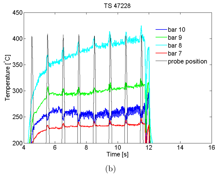
Figure 4.11: (a) Infra-red image of ICRH antenna equipped with the new type of FS. (b) Temporal evolution of the surface temperature measured on selected bars located in the bottom right quarter. The probe is not connected to the bars, it just passes \approx 1\text{cm} in front of them. By black color is superimposed the probe position.
