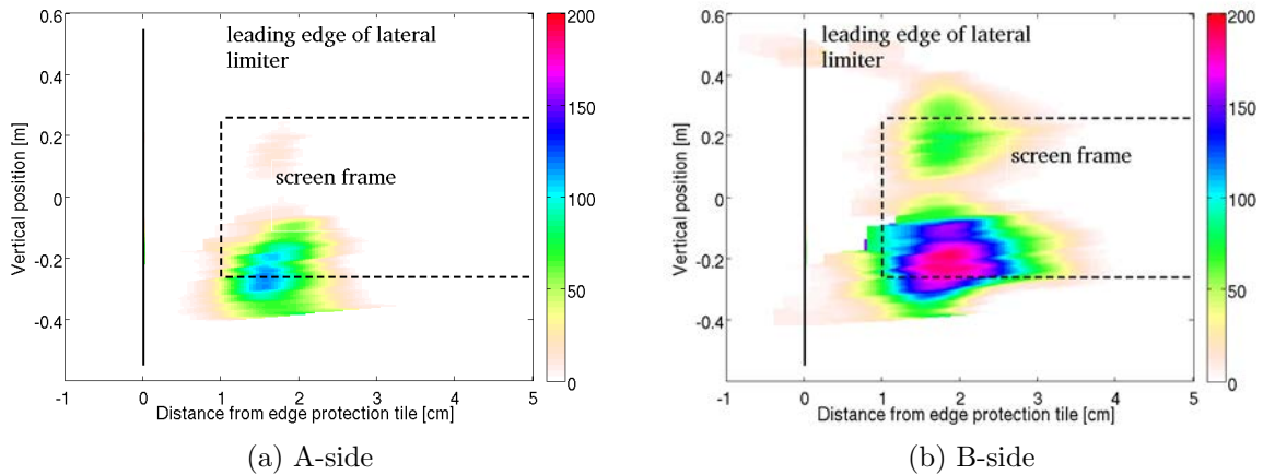
Figure 5.12: Detailed 2D map of floating potential measured on flux tubes unconnected (a) and connected (b) to powered ICRH antenna equipped with the new FS.
