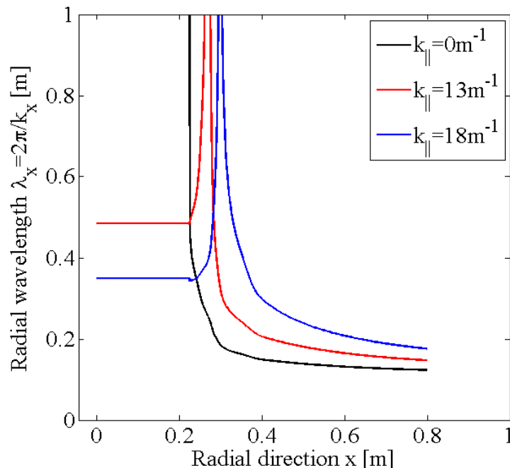
Figure 4.6: Radial wavelength \lambda_x (in m) versus the radial direction x (in m) pointing towards the plasma center for different characteristic values in the antenna k_{||} spectrum: minimum value, optimal value and maximum value.
