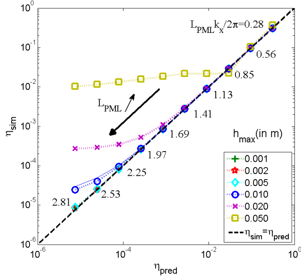
Figure 3.4: Comparison of the reflection coefficient obtained in the simulations with the expected analytical reflection coefficient during a scan of the PML depth L_{PML} for several maximum element size parameters h_{max\perp} with a mapped regular mesh. The curve \eta_{sim} = \eta_{pred} is also plotted as a reference. Each dot represents one simulation. An example with a triangular mesh is also shown with cyan circles.
