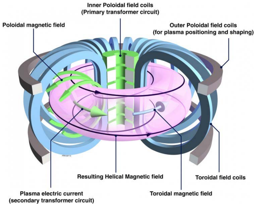
Figure 1.1: Schematic view of the tokamak concept.
