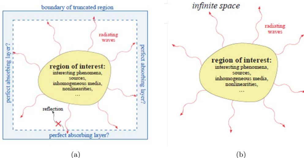
Figure 2.5: A finite region of interest where sources, inhomogeneous media, non-linearities are being investigated. (a) Sketch of a typical bounded wave-equation problem. An absorbing layer is placed adjacent to the edges of the computational region to absorb outgoing waves without reflection coming from the edge of the absorber. (b) Sketch of a typical unbounded wave-equation problem that we want to solve as exactly as possible to reality. Courtesy of Steven J. Johnson [79]
