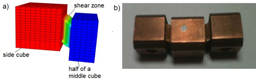
Figure 3.16: a) Half of a deformed specimen - numerical prediction, b) deformed specimen after experiment.
