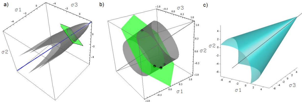
Figure 4.1: The yield surfaces in the space of principal stresses (\sigma_1, \sigma_2, \sigma_3) : a) a paraboloid of revolution - the Burzyński criterion, b) a cylinder of revolution - the Huber-Mises-Hencky criterion, c) a cone - the Drucker-Prager criterion. All three cases are detailed formulation of the Burzyński hypothesis.
