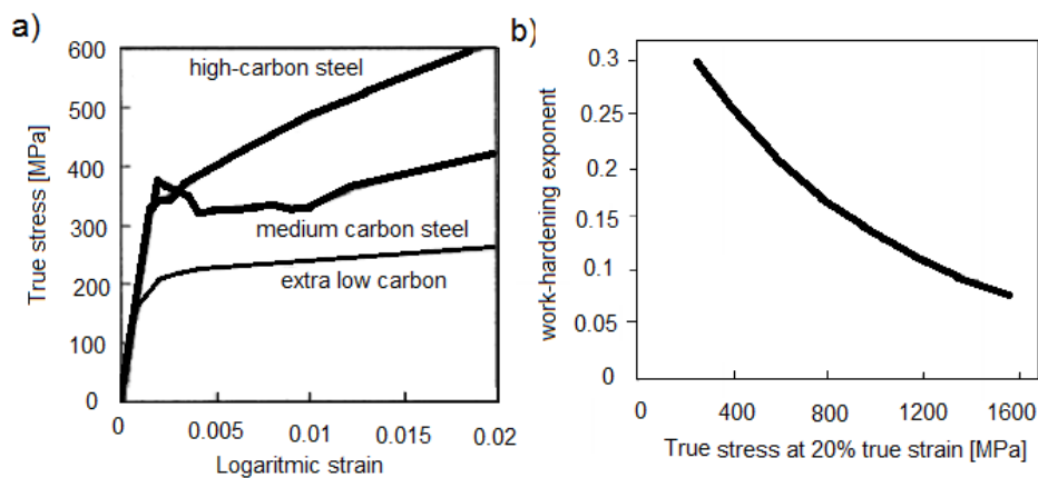
Figure 2.8: Stress-strain curve dependence on carbon content in ferritic steels, b) work-hardening exponent dependence on steel strength, [Kostryzhev 2009; Akiyama et al. 2002].
