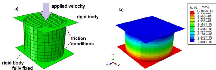
Figure 3.8: a) Boundary conditions of a quasi-static compression test, b) deformed mesh for the frictionless conditions.
